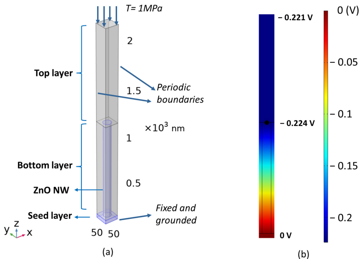
Figure 4. COMSOL model of ZnO NW: (a) schematic structure of a unit cell consisting of ZnO SL, bottom matrix layer, top matrix layer, and single ZnO NW with proper boundary conditions; (b) electric potential longitudinal profile of unit cell subjected to an axial compression (viewed in 2D YZ cut plane).
