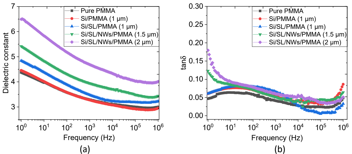
Figure 15. Variation of the (a) dielectric constant, and (b) loss tangent as a function of the frequency of different samples.
