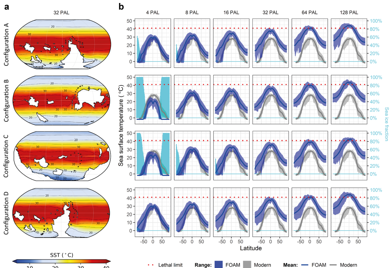
Fig. 4 FOAM GCM simulations of early Cambrian sea-surface temperatures for each continental configuration (A–D) with present-day orbital parameters. a Maps of simulated SST for configurations A–D at 32 PAL p\text{CO}_2 . b Zonally averaged model (dark blue) SST annual mean and seasonal variation for each configuration and p\text{CO}_2 forcing, with comparable present-day SST values (grey) from ref. 72 , and lethal temperature limit for animals of 41 °C, following ref. 50 , plotted with mean zonal sea-ice cover (light blue). The sea ice cover represents the percentage of the ocean that is covered by sea ice (yearly average). p\text{CO}_2 levels relative to PAL (=280 ppm).
