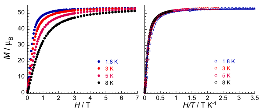
Fig. 5. Field dependence of the magnetization, M , for 3 below 8 K plotted as (left) M vs H and (right) M vs H/T plots. The solid blue line is the best fit of the M vs H/T plots to a sum of the S = 12 and S = 29/2 Brillouin functions (with g = 1.99(2) ) as discussed in the text.
