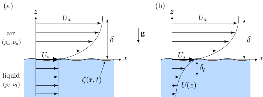
FIG. 1. Flow configuration. A liquid is subject to a turbulent air flow blowing at its surface with velocity U_a . The liquid is characterized by its density \rho_l , viscosity \nu_l , and surface tension \gamma . The air turbulent boundary layer is characterized by its density \rho_a , kinematic viscosity \nu_a , boundary layer thickness \delta , and friction velocity u^* . Fluctuations in the surface elevation \zeta(\mathbf{r}, t) result from the turbulent stresses applied at the interface. Two current configurations are illustrated: (a) uniform current of constant velocity U_s and (b) exponential velocity profile of thickness \delta_l . Both cases are illustrated here in the case \theta = 0 (current aligned with the wind direction). The velocity profiles are not drawn to scale: the velocity in the air is typically 20 times larger than that in the liquid.
