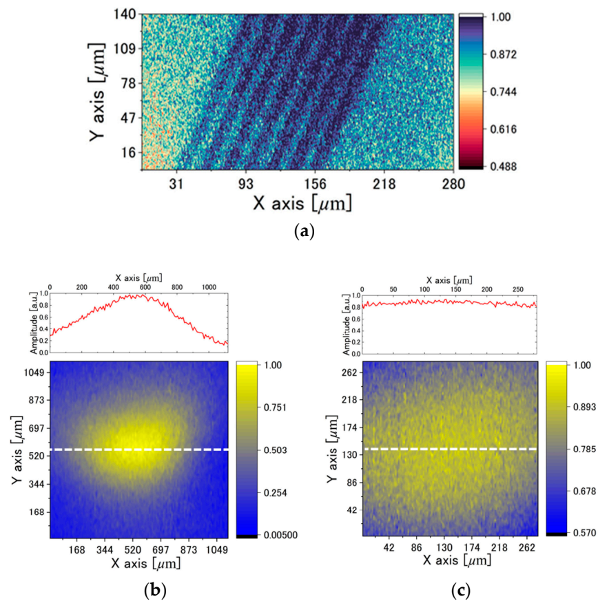
Figure 2. (a) Terahertz reflection image of 9 \mu\text{m} gold interdigitate structure. (b,c) Terahertz transmission images when no samples are set on the GaAs crystal in a size of wide (1.1 mm \times 1.1 mm) and narrow (280 \mu\text{m} \times 280 \mu\text{m} , Field of view) scanning mode with a line profile along the white dashed line inserted in each image.
