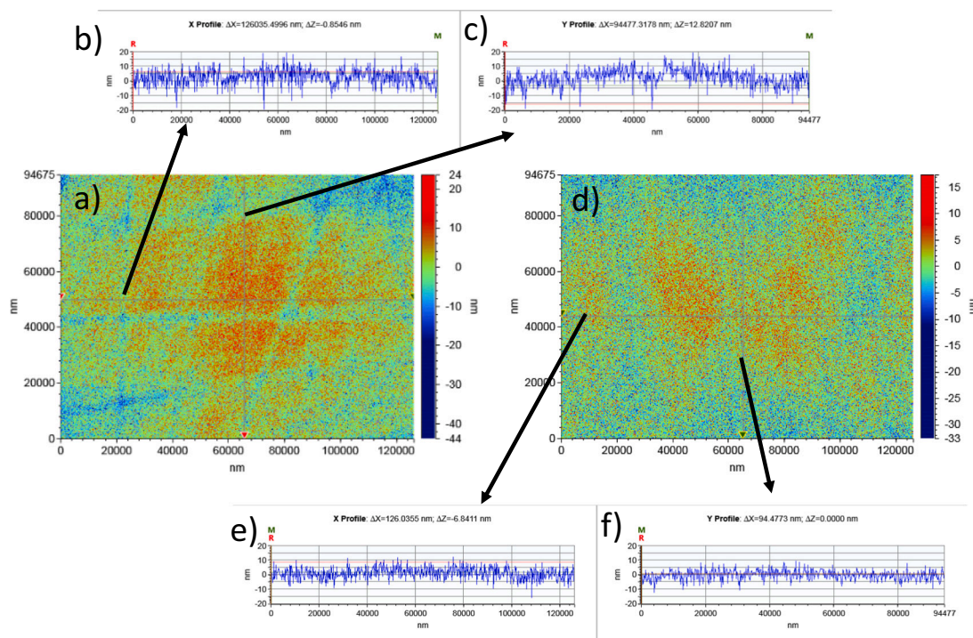
Fig. 2. Roughness mapping of (a) \text{TiO}_2 film and (d) TiN film, obtained by interferometric confocal microscopy; (b–c) extracted X and Y profiles for the \text{TiO}_2 film; (e–f) extracted X and Y profiles for the TiN film.
