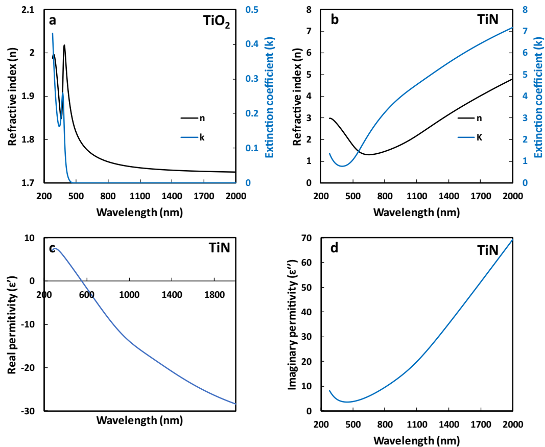
Fig. 5. Refractive index ( n ) and extinction coefficient ( k ) according to the wavelength (Vis-NIR) for (a) TiO 2 thin film and (b) TiN. Permittivity according to the wavelength for TiN film: (c) real part ( \epsilon' ) and (d) imaginary part ( \epsilon'' ).
