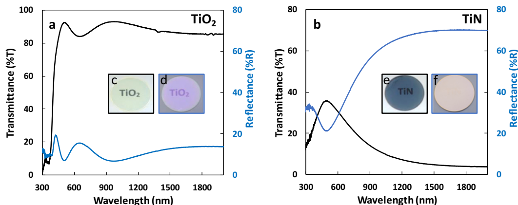
Fig. 4. UV-Visible-NIR reflectance and transmittance spectra of (a) TiO 2 and (b) TiN thin film. Inset (c) and (d): optical photographs of TiO 2 thin films in transmission and specular reflection, respectively. Inset (e) and (f): optical photographs of TiN thin films in transmission and specular reflection, respectively.
