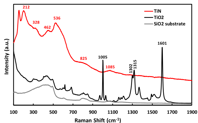
Figure 2. Raman spectra of a bare glass substrate ( \text{SiO}_2 ), \text{TiO}_2 , and \text{TiN} thin films.
