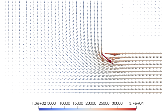
Fig. 8. Current density distribution in the corner of the external turn of the bottom layer copper trace (in A/m^2 ) at 100 kHz.
