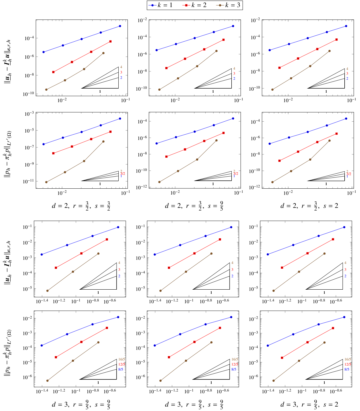
Figure 1: Numerical results for the test cases of Section 5.1 where \frac{r^*}{r} = 2 . The slopes indicate the convergence rates expected from Theorem 17 when s = 2 , and [11, Theorem 12] otherwise.
