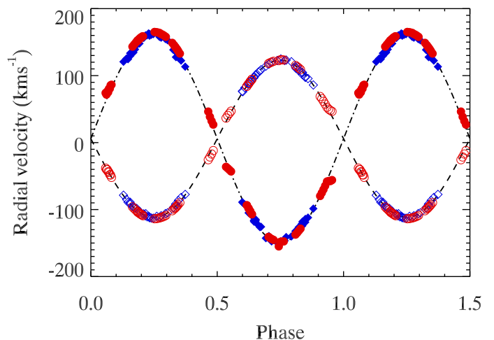
Fig. 2. Orbital solution obtained for the two components of UV Psc. The circles (red) correspond to our observations with ESPaDOnS in 2016, the diamonds (blue) are measurements by Popper (1997). Filled symbols represent radial velocities for UV Psc B. The best-fitting orbits for the primary and secondary are indicated with the dashed and dash-dotted lines, respectively.
