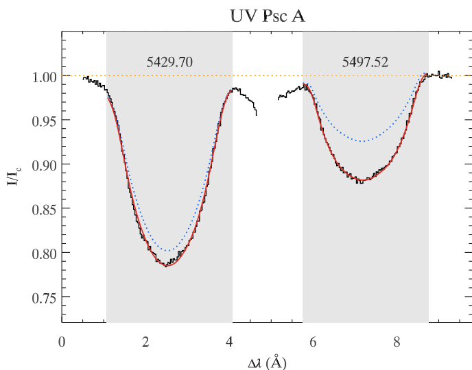
Fig. 11. Profiles of the two Fe I spectral lines employed for inferring the magnetic field strength for UV Psc A. Observations are shown in black histograms and are compared to the median parameter fit (red solid line). The blue dotted lines correspond to the non-magnetic synthetic spectrum. The dark grey areas indicate the wavelength regions where the fitting has been carried out.
