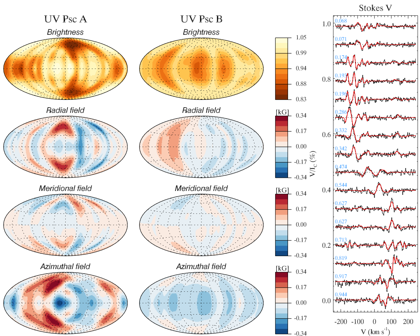
Fig. 5. Left. Maps of the brightness distribution (top row), obtained from the Stokes I spectra and the magnetic field components (row 2–4), obtained from the Stokes V spectra for UV Psc A (left column) and UV Psc B (right column). The surface is represented using the Hammer-Aitoff projection in order to preserve the relative area of different latitude bands. The central meridian corresponds to a longitude of 180^\circ . The substellar points are located at the longitude 0^\circ for UV Psc A and at 180^\circ for UV Psc B. The colour bars on the right indicate the relative surface brightness and magnetic field strength in kG for each map. Right. Observed (black histogram) and best-fit spectra (red solid lines) obtained from the ZDI analysis. The spectra for different phases are offset vertically, with the phase indicated next to each spectrum.
