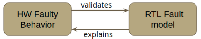
Fig. 6. Relation between hardware faulty behaviour and RTL fault model.
