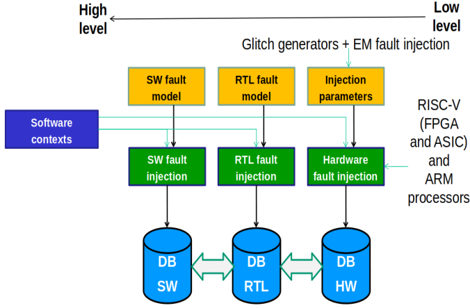
Fig. 5. Proposed Methodology.
