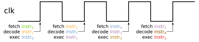
Fig. 1. Normal behaviour with a regular clock signal.
