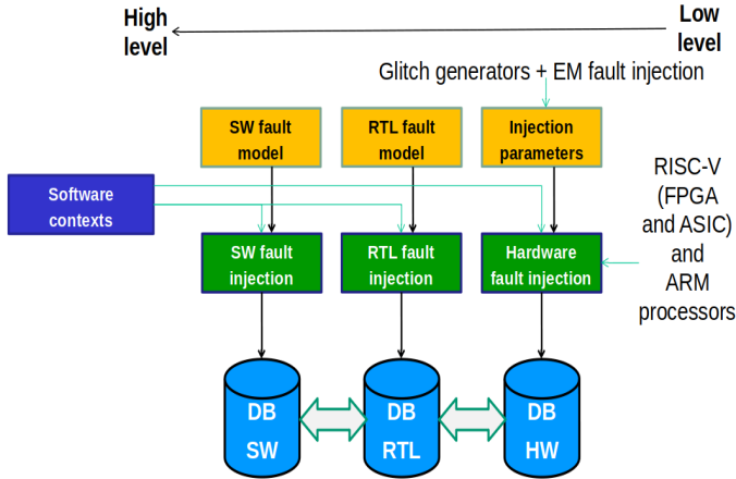
Fig. 5. Proposed Methodology.
