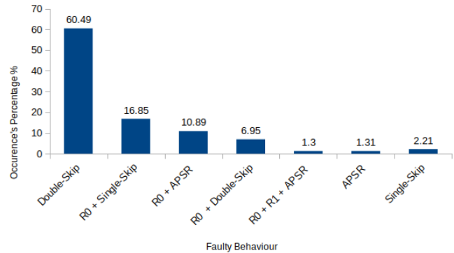
Fig. 3. Observed faults after the first campaign
