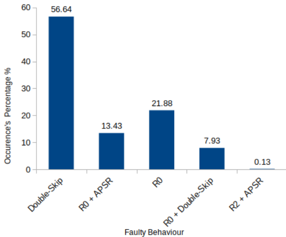
Fig. 4. Observed faults after the second campaign
