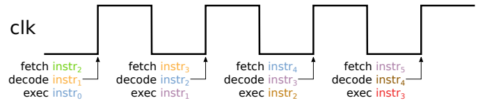
Fig. 1. Normal behaviour with a regular clock signal.
