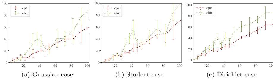
Fig. 10: Evolution of the SHD for CBIC (dotted green line) and CPC (dot-dashed red line) methods with respect to the dimension of the random graphs. The results are averaged over 2 different random graphs of the same dimension and over 5 different data sets of size M = 10000 .
