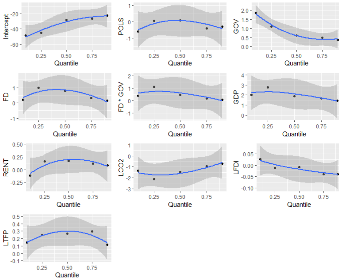
Fig. 1. Quantile process coefficient estimation with 95% confidence intervals Powell (2016).
