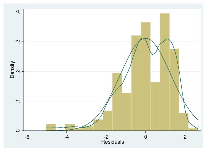
Figure A2. Residuals distribution.
