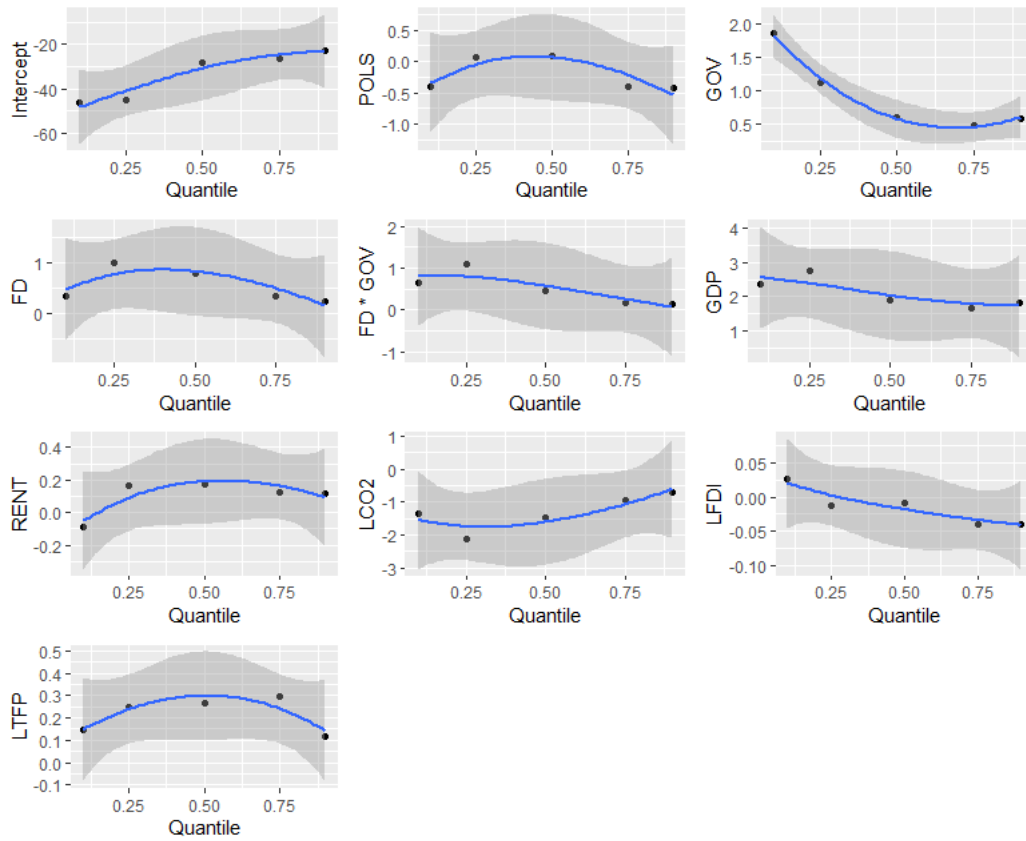
Fig.2. Quantile process coefficients estimation with 95% confidence intervals (Canay's (2011) fixed-effect quantile model)
