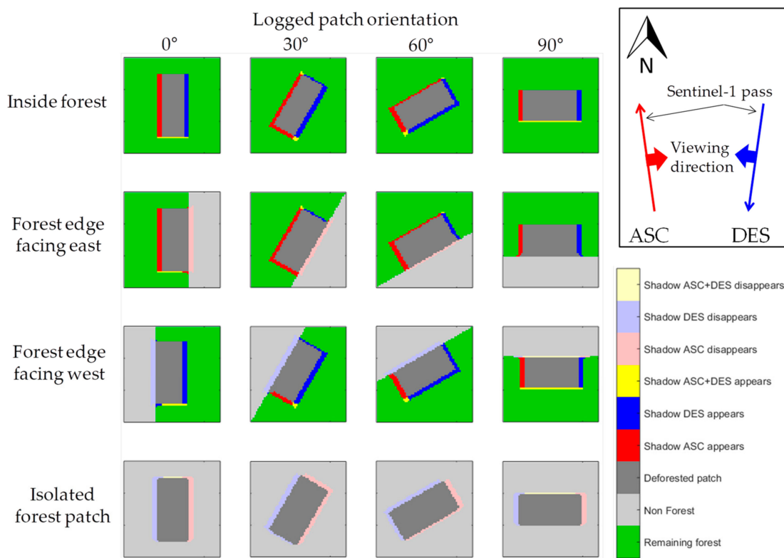
Figure 4. Shadows that appear or disappear when a forest patch is deforested, depending on the orbit orientation (ascending or descending), the patch orientation, and the configuration (patch inside a forest, at the edge of a forest, or isolated). The figure is simulated for the Sentinel-1 configuration (right-looking with 98.18^\circ orbit inclination) which is summarized in the frame on the top right.
