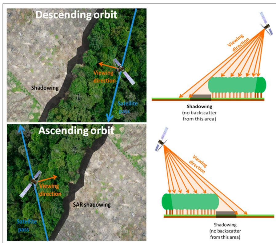
Figure 3. Illustration of the synthetic aperture radar (SAR) shadowing effect at the border between forests and deforested areas, for the descending and ascending orbit configurations. (Background image: ConservationDrones.org/Orangutan Conservancy.)
