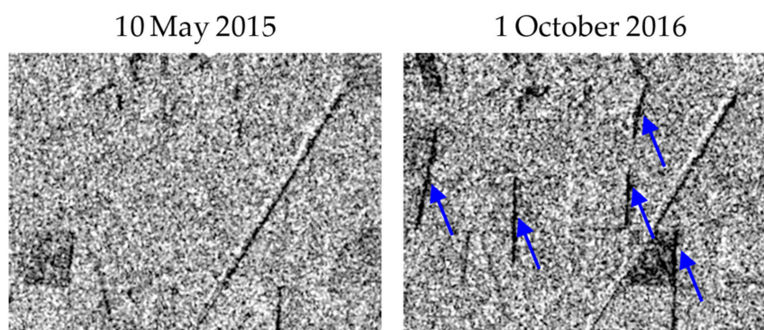
Figure 6. A 2.6 \text{ km} \times 3.4 \text{ km} subset of Sentinel-1 intensity images acquired in descending orbit on 10 May 2015 and 1 October 2016 over a rubber plantation area, centered on 11^{\circ}16'40''\text{N} 106^{\circ}39'40''\text{E} . Blue arrows indicate shadows that appear between the two dates because of harvest.
