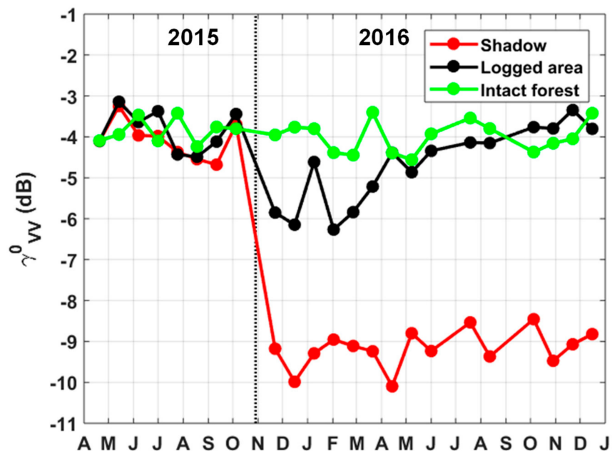
Figure 5. Temporal backscatter profiles of an area being logged (black), the corresponding shadow (red) that is created on one of its edges when deforestation occurs (October–November 2015), and an intact forest (green).
