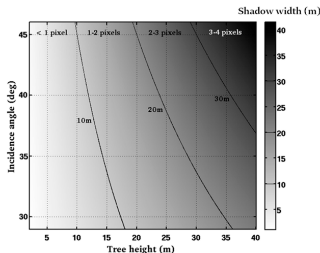
Figure 7. Shadow width as a function of tree height and Sentinel-1 incidence angle. The corresponding number of pixels is based on a 10 m pixel size.
