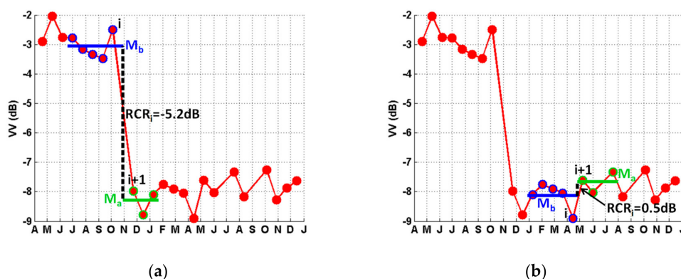
Figure 8. Temporal variation of the VV backscatter in an area detected as a new shadow (red), and illustration of the calculation of the change indicator \text{RCR}_i (radar change ratio) for X_b = 5 and X_a = 3 for two pairs of dates: (a) the exact date interval during which change occurs; (b) a date interval when no change occurs.
