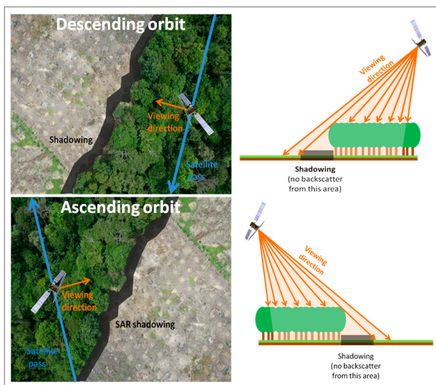
Figure 3. Illustration of the synthetic aperture radar (SAR) shadowing effect at the border between forests and deforested areas, for the descending and ascending orbit configurations. (Background image: ConservationDrones.org/Orangutan Conservancy.)
