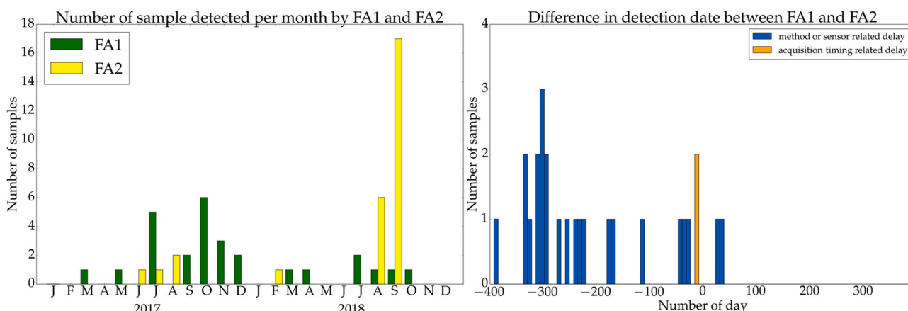
Fig. 10. Regarding forest exploitation: number of detected reference samples per month for FA1 (green) and for FA2 (yellow) Forest Alerts systems (left), and histogram of the difference in detection date of the reference samples (right), where negative values indicate an earlier detection in FA1. (For interpretation of the references to colour in this figure legend, the reader is referred to the web version of this article.)
