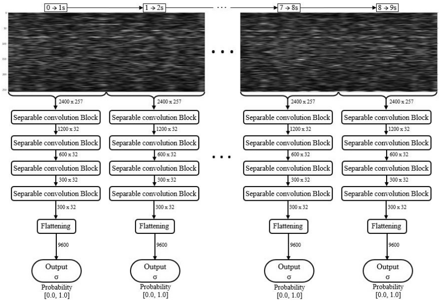
Fig. 1: SepaConvNet architecture.
