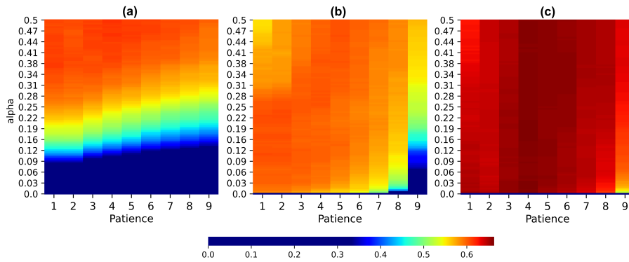
Fig. 2: Final BTQ of the three comparative methods at the end of the 9 second MER signal averaged across all k folds of cross-validation. Adaptive Listening time with SepaConvNet (a), the Simple Bayesian Extension (b), and the Advanced Bayesian Extension (c).
