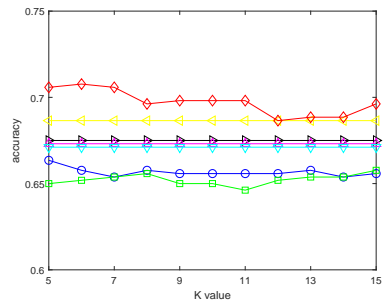
(l) Sonar with n = 20
