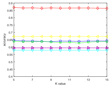
(i) Parkinson with n = 8
