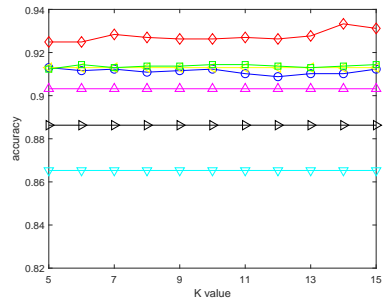
(c) Wdbc with n = 10
