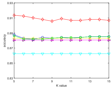
(f) Ionosphere with n = 10
