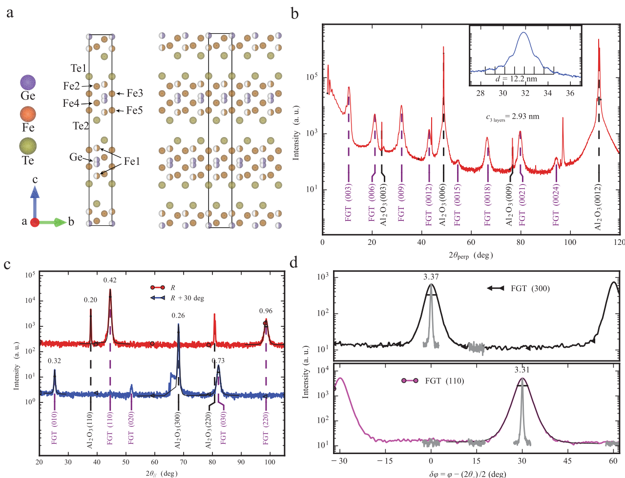
Fig. 2 Structural characterization of Fe 5 GeTe 2 by X-ray diffraction. a Unit cell projected along [100], with FGT layers separated by the vdW gap between adjacent Te sublattices. The right-side image shows the same projection for several repetitions of the unit cell. The occupation probability is represented by half-filled solid balls. Images generated using VESTA software 52 for the crystallographic model of ref. 7. b Out-of-plane \theta/2\theta XRD scan of the films, showing Al 2 O 3 (00 l ) and Fe 5 GeTe 2 (00 l ) peaks. Inset: zoom on the (009) Bragg peak to show the fringes used to estimate the film thickness. c In-plane radial XRD scans along the (110) reciprocal direction ( R ), and (010), ( R+30^\circ ). Each diffraction peak is labelled with the full width at half maximum. d In-plane azimuthal XRD scan over the families {110} and {300} showing the 6-fold symmetry of the crystal. Grey lines show the corresponding radial peak.
