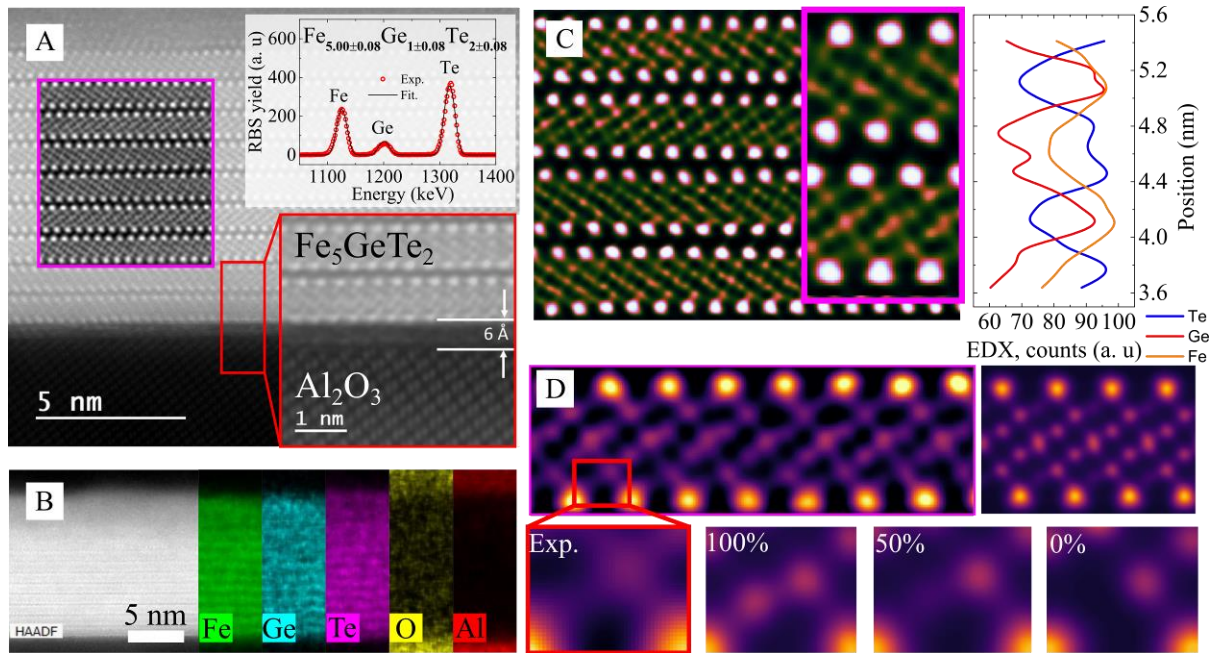
Figure 3 Transmission electron microscopy of Fe_5GeTe_2 . (A) High-angle annular dark-field (HAADF) cross section image of the 12 nm-thick film along [110]. Left inset: High-pass filtered image of the layers. Top inset: Rutherford backscattering spectroscopy showing stoichiometric 5:1:2 Fe:Ge:Te composition. Bottom inset: Zoomed view of the interface between Al_2O_3 and Fe_5GeTe_2 . (B) Element distribution across the layers, determined using energy dispersive X-ray spectroscopy (EDX). (C) Atomic number contrast enhanced HAADF image of the Fe_5GeTe_2 layers. The left plot shows an EDX scan over two layers, selective to Te, Ge, and Fe. (D) Comparison between experimental (top left panel) and simulated (top right panel) Z-contrast enhanced HAADF images. Bottom panels are zooms on the Fe1 site. The simulations consider different occupation probabilities of the Fe1 site.
