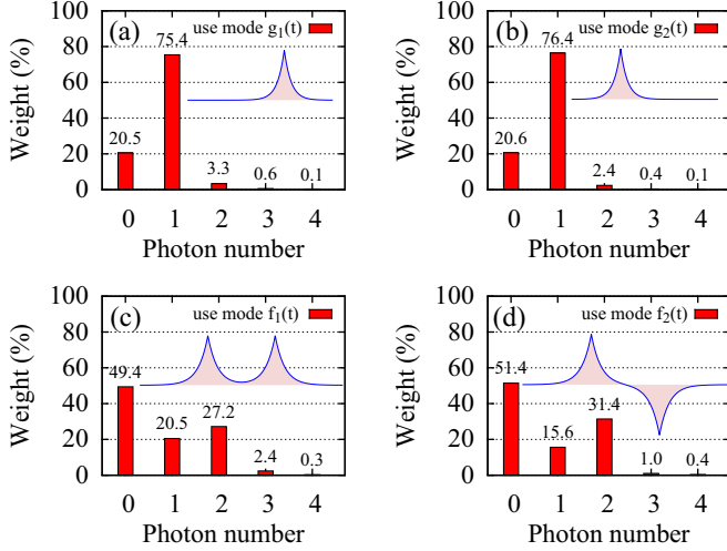
FIG. 4. Photon-number distributions of the reconstructed states for the different temporal-mode functions g_1(t) , g_2(t) , f_1(t) , and f_2(t) shown in the insets. The distributions are not corrected for detection losses. The delay is set to 40 ns.
