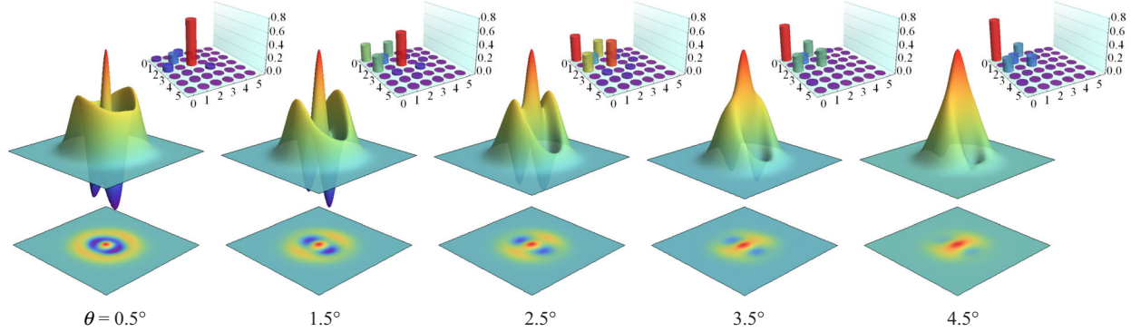
FIG. 3 (color online). Experimental results. The plots give the density matrices (absolute values) and the associated Wigner functions for incremental values of the half-wave plate angle \theta ( \epsilon between 0.017 and 0.16). The results are corrected for the \eta = 85\% detection efficiency. For \theta = 1.5^\circ , the negative peaks of the Wigner function reach W = -0.27 \pm 0.01 .
