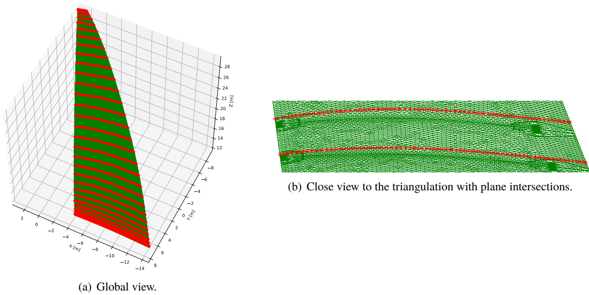
Figure 4: Mainsail triangulation.
