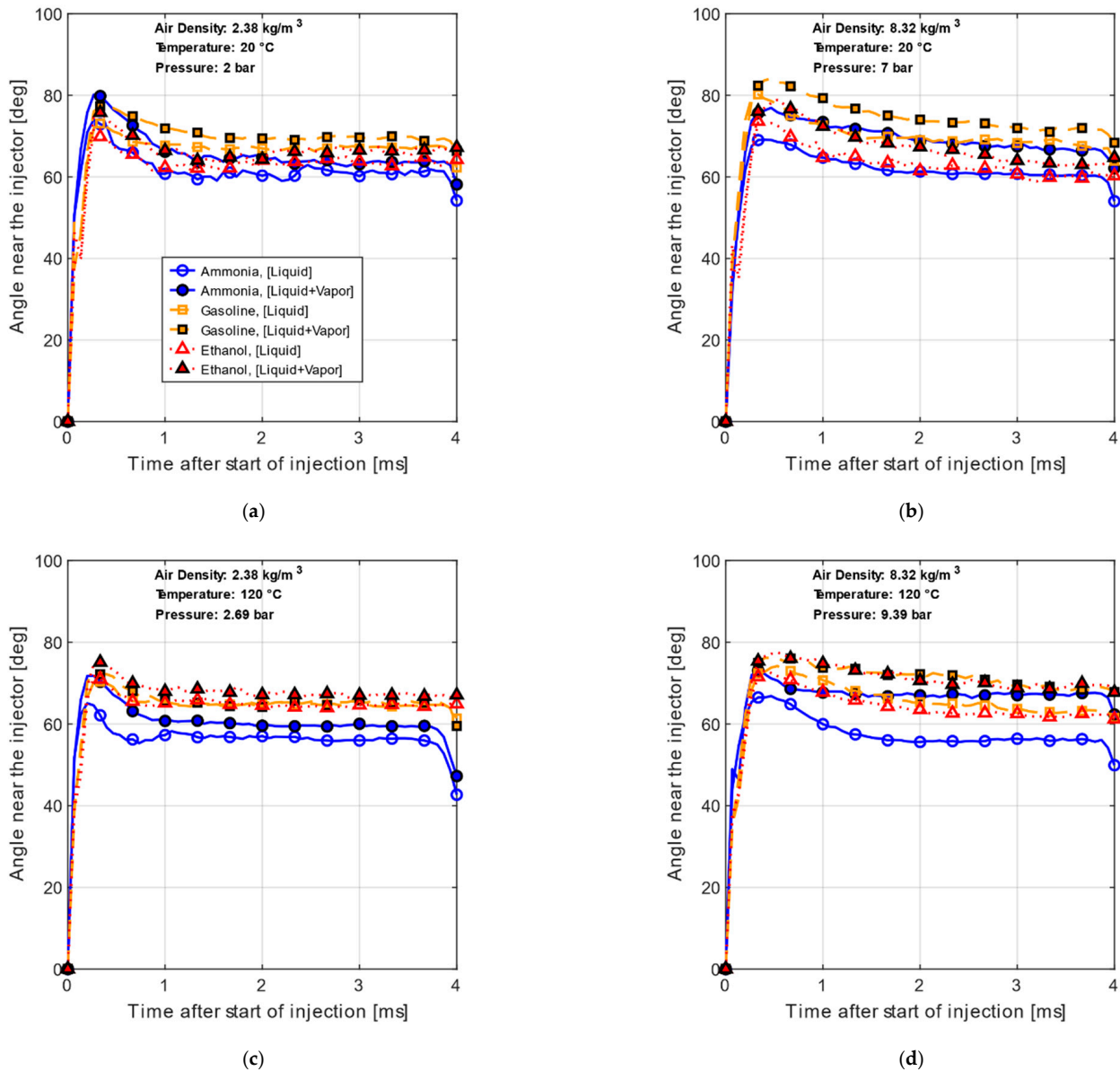
Figure 7. Comparison of spray angle near the injector for ammonia (continuous line), gasoline (dashed line) and ethanol (dotted line), (a) T_{air} = 20\text{ °C} and P_{air} = 2\text{ bar} , (b) T_{air} = 20\text{ °C} and P_{air} = 7\text{ bar} , (c) T_{air} = 120\text{ °C} and P_{air} = 2.69\text{ bar} , and (d) T_{air} = 120\text{ °C} and P_{air} = 9.39\text{ bar} .
