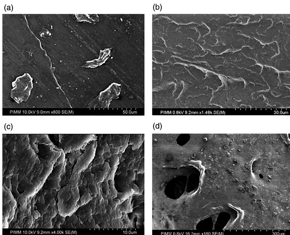
FIGURE 3 Micrographs of scanning electron microscopy (SEM) observations of wastes of electrical and electronic equipment (WEEE) acrylonitrile-butadiene-styrene/polycarbonate (ABS/PC) blends: (a) ABS/PC (100/0) fractured surface, (b) ABS/PC (70/30) fractured surface, (c) ABS/PC (30/70) fractured surface, (d) ABS/PC (30/70) after dissolution in acetone
