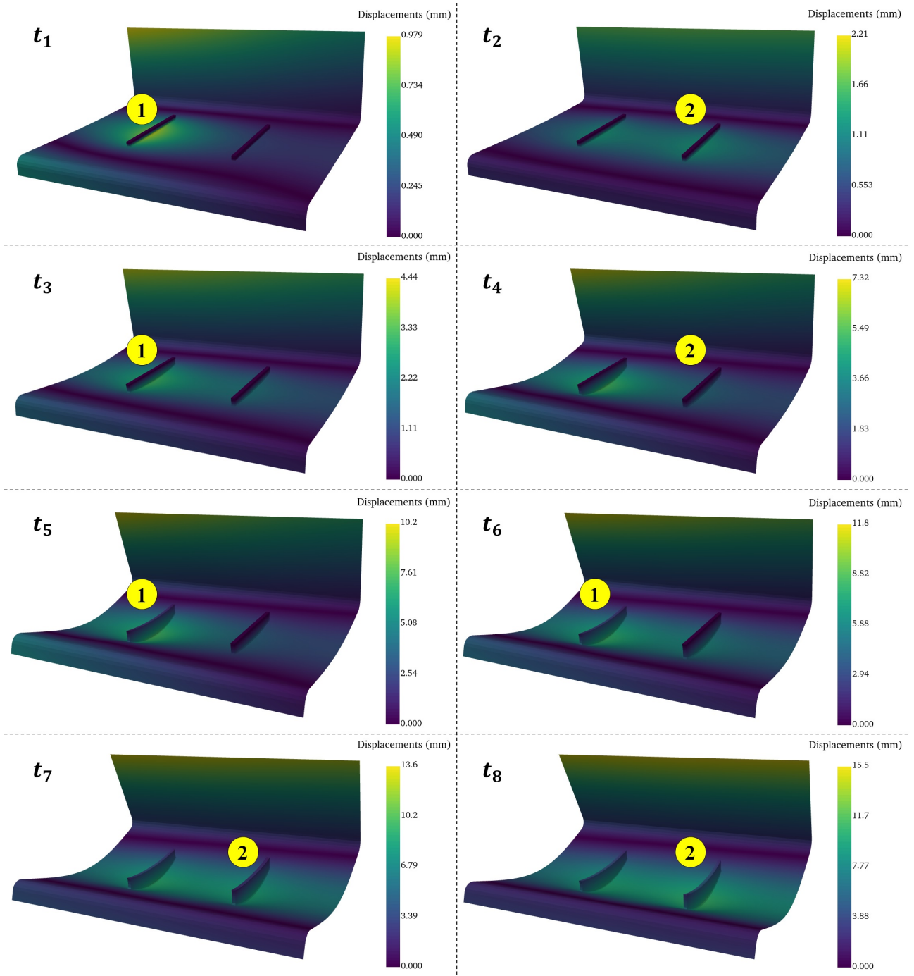
Figure 5. High-fidelity simulation of the sequence \{1, 2, 1, 2, 1, 1, 2, 2\} (displacements \times 3 for visualization). Both stiffeners are placed from the beginning on the sheet, and each layer of them is sequentially mechanically activated.
