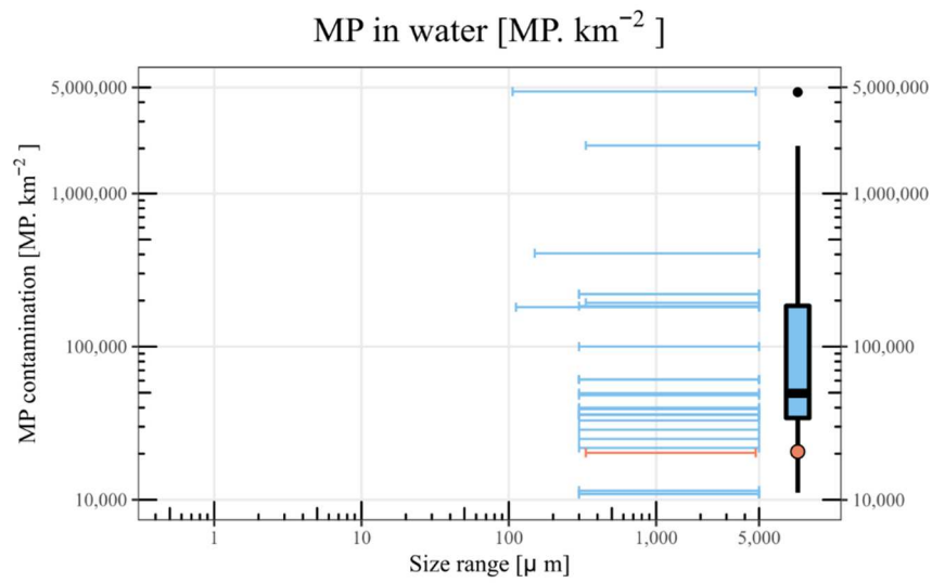
2 Fig. 1. Microplastic concentrations on surface waters of worldwide lakes ( \text{MP}/\text{m}^3 or \text{MP}/\text{km}^2 ) according to size 3 range studied and anthropogenic pressure (rural, urban)
