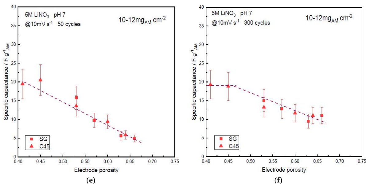
Figure 4. Specific capacitance vs. electrode porosity of the \alpha -MnO 2 symmetric supercapacitor device using SG or C45 carbon black additive, after cycling in 5M LiNO 3 at 10 mV·s -1 : (a) Low-mass loading, 50 cycles; (b) Low-mass loading, 300 cycles; (c) Medium-mass loading, 50 cycles; (d) Medium-mass loading, 300 cycles; (e) Large-mass loading, 50 cycles; (f) Large-mass loading, 300 cycles. Dashed lines are guidelines for the eyes.
