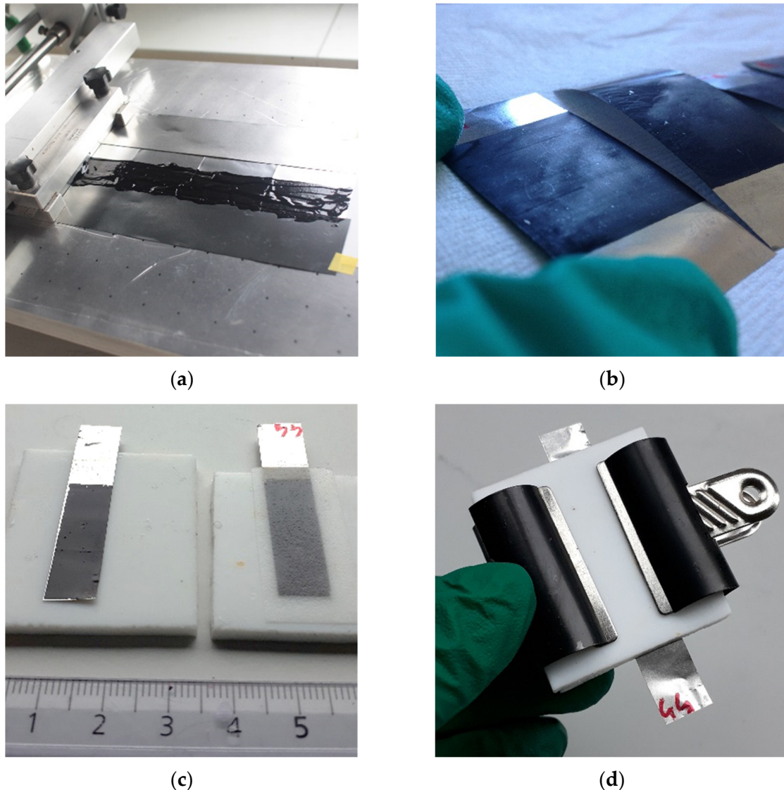
Figure 1. Fabrication steps of \alpha\text{-MnO}_2 ink electrodes and the symmetric device: (a) Ink coating using a doctor blade apparatus; ink containing a dry matter of c.a. 25 wt.% is coated on stainless steel current collectors; the gap between the doctor blade and the substrate can be adjusted in order to prepare \text{MnO}_2 -based electrodes with different mass loadings; (b) After drying at 60\text{ }^\circ\text{C} for 1 night under vacuum for 1–2 h, the coated stainless steel substrate is cut into rectangular-shaped electrodes; (c) Electrodes are assembled according to a face-to-face two-electrode design; the two electrodes are separated by a cellulosic separator impregnated with 5M \text{LiNO}_3 neutral aqueous electrolyte and the stack is pressed between two Teflon ® plates; (d) \alpha\text{-MnO}_2 symmetric two-electrode cell; the metallic clamps enable the application of the same pressure to all the symmetrical devices.
