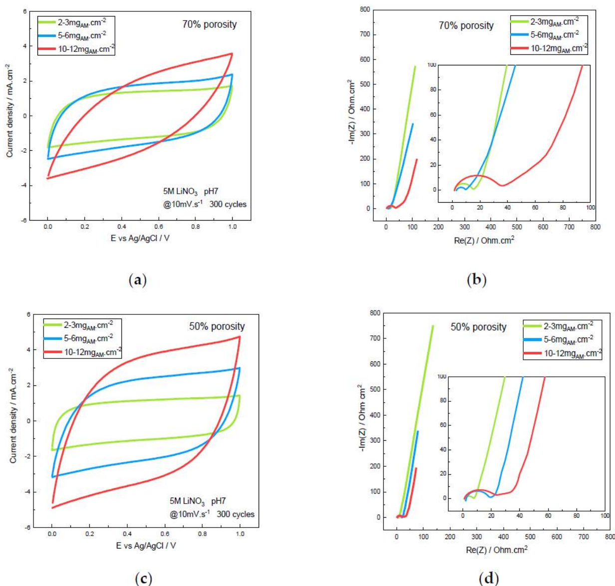
Figure 7. Cyclic voltammetry and electrochemical impedance spectroscopy of the \alpha - \text{MnO}_2 symmetric supercapacitor device after 300 cycles in 5M \text{LiNO}_3 at 10 \text{ mV} \cdot \text{s}^{-1} for low-, medium- and large- mass loading at two different porosities: (a) 70% porosity, CV; (b) 70% porosity, Nyquist diagram (200 kHz–2 mHz at E_{OC} , 20 mV potential amplitude); (c) 50% porosity, CV; (d) 50% porosity, Nyquist diagram (200 kHz–2 mHz at E_{OC} , 20 mV potential amplitude) (inserts: magnification of the Nyquist diagrams).
