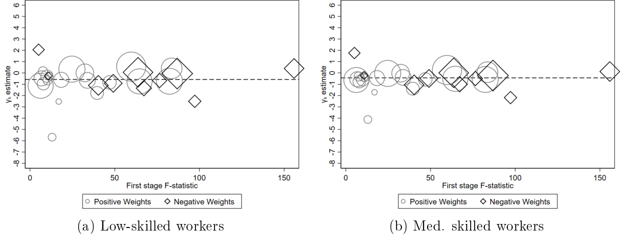
Figure A1: Distribution of Rotemberg Weights for each skill
