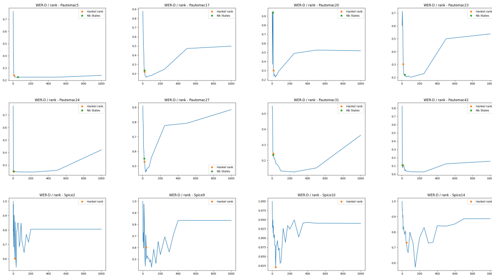
Figure 8: Evolution of the quality in term of WER-D on S_{RNN} with the value of the rank hyper-parameter on some PAutomac and SPiCe problems (basis size is 1000 prefixes and suffixes).
