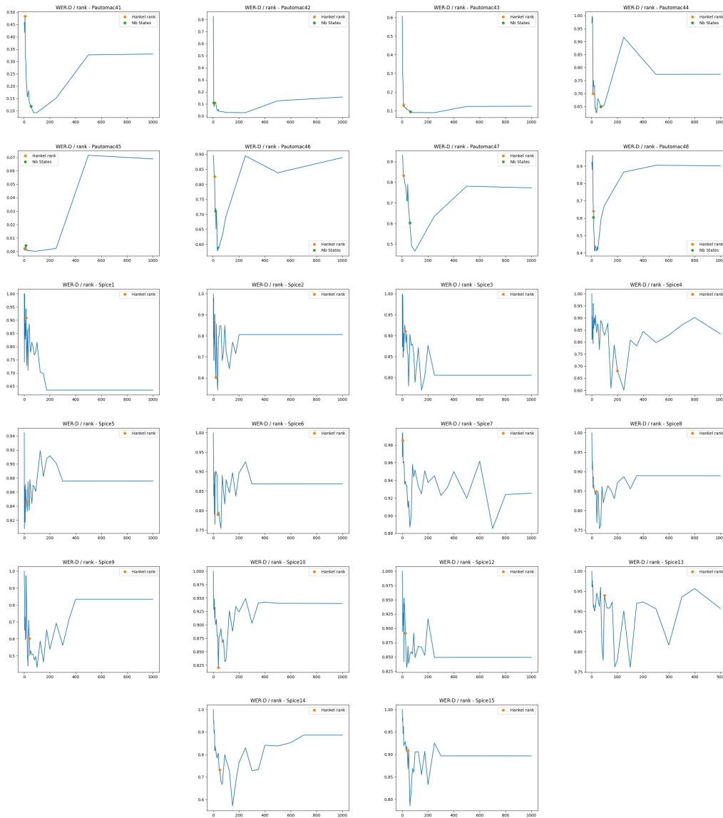
Figure 10: Evolution of the quality in term of WER-D with the value of the rank hyperparameter on the 8 last PAutomaC problems and the SPiCe ones, evaluated on S_{RNN} with basis size 1000 \times 1000 .
