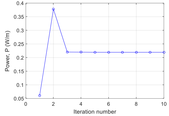
Fig. 6. Evolution of the power dissipated in the iterative solving ( \varepsilon=10^{-6} )
