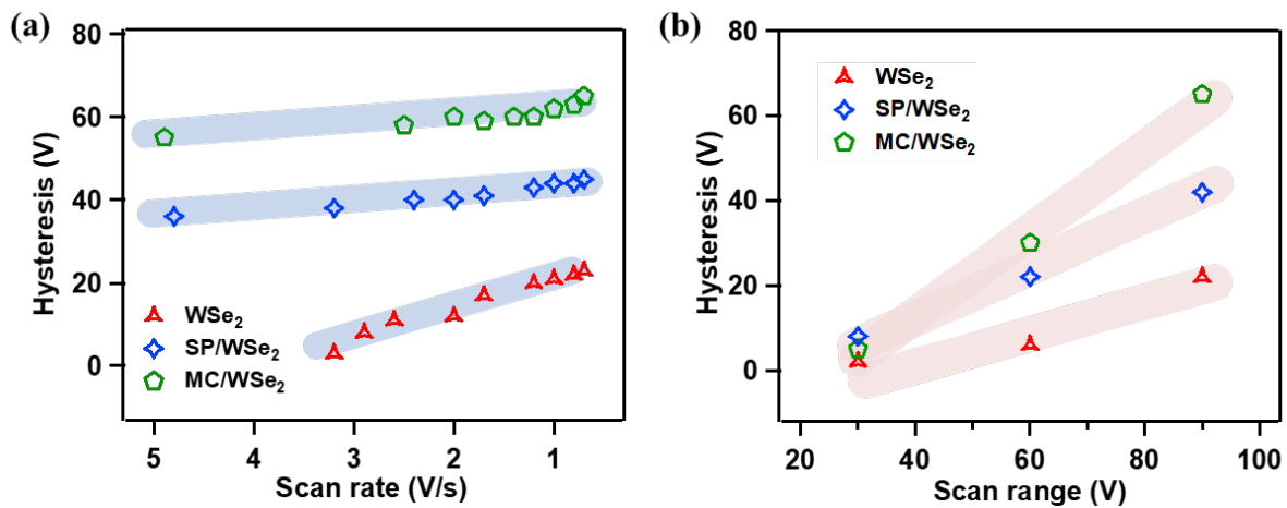
Figure 5. Hysteresis characterization. (a-b) Hysteresis comparison of FETs based on bare WSe_2 , SP/WSe_2 and MC/WSe_2 under (a) different scan rates, (b) different scan ranges.
