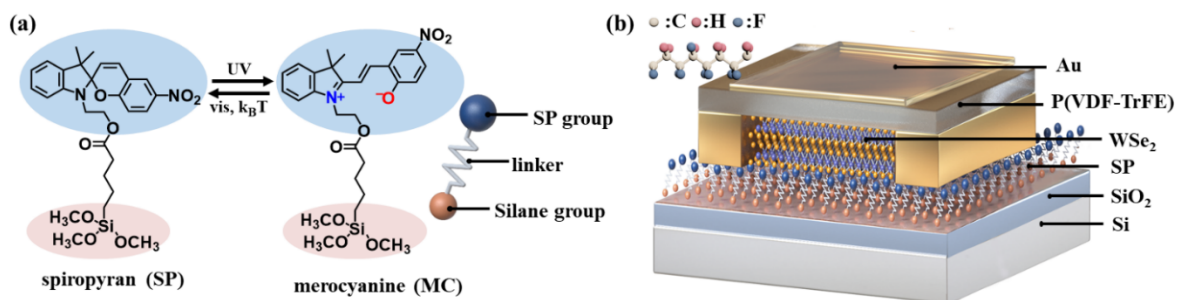
Figure 1: (a) Structure formulae of SP and MC and scheme of the SP – MC reversible isomerization obtained upon irradiation with UV ( \lambda = 365 nm) and vis ( \lambda = 530 nm) light, respectively. (b) Schematic illustration of the Janus SP/WSe 2 /P(VDF-TrFE) FET device with double-sided decoration: the bottom surface of WSe 2 is functionalized with SP SAM and the top surface is functionalized with P(VDF-TrFE) layer.
