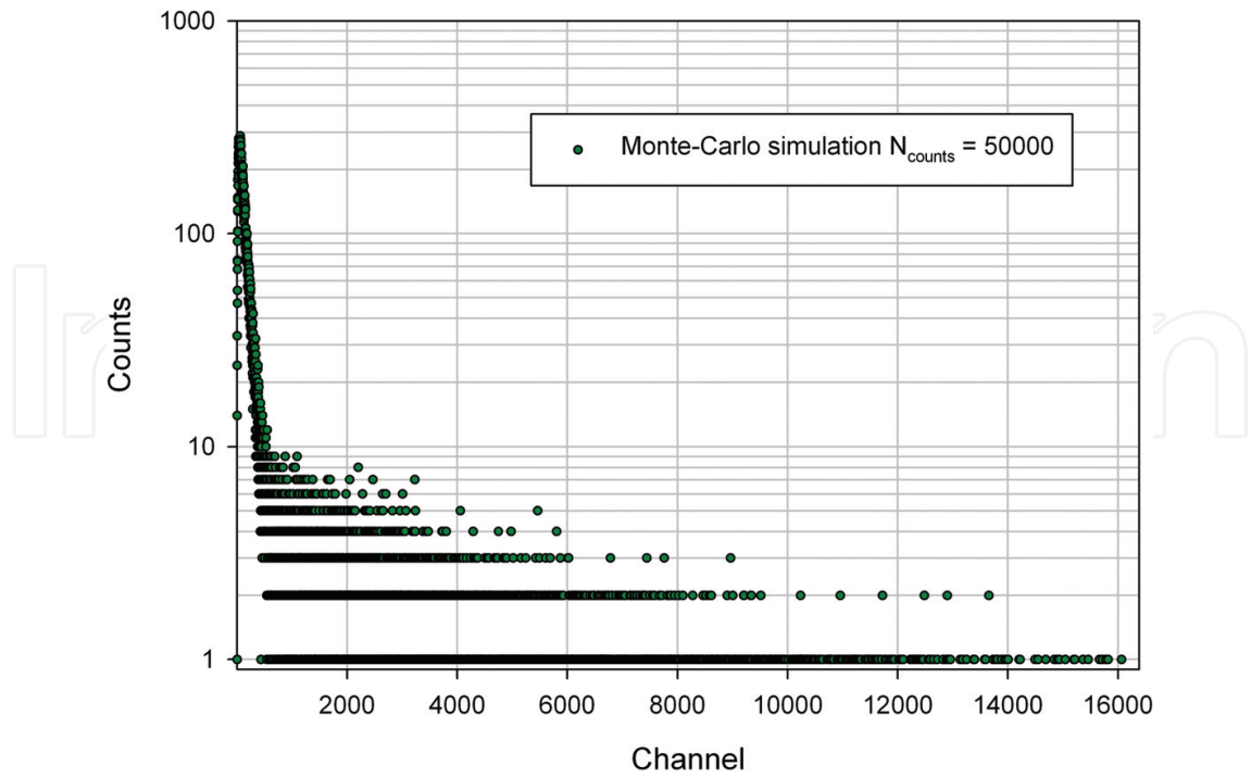
Figure 7. Simulated histogram of the VUV fluorescence ( N_C , 16,384; R , 5 ns).
