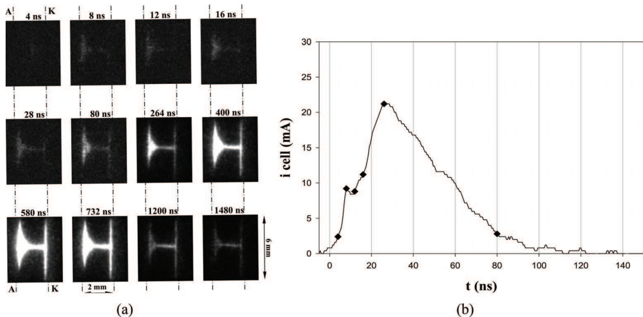
Figure 13. The micro-discharge for P_{\text{Xe}} 200 Torr; f , 10 kHz; d , 2 mm; and U_{\text{max}} , 2.36 kV. (a) Evolution of the micro-discharge: 3 ns exposure time snapshots in the visible range (360 to 920 nm). The 264 ns snapshot is the reference for light intensity. A, anode; K, cathode. (b) Cell current with expanded time scale. Rhombuses correspond to the first six snapshots of (a) [36].
