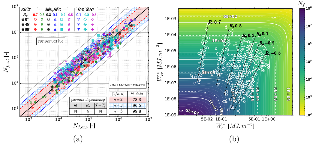
Figure 22: Performance of the proposed criterion based on the creep and cyclic energies: (a) comparison between the predicted fatigue life and the experimental one, (b) shape of the fatigue iso-lifetime.
