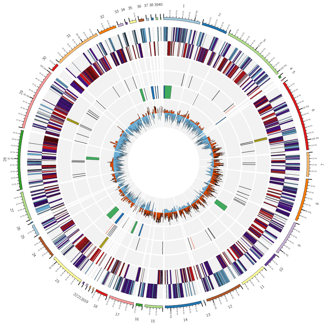
FIGURE 1 | Circular diagram of LsoD ISR100 genome. Descriptions of rings are from the outer to inner circle. (i) Contigs; (ii) protein coding genes in the positive (blue) and negative (red) strands. Enzymes in both strands are highlighted in purple; (iii) rRNA genes (yellow); (iv) tRNA (black lines) and other non-coding RNA (red lines); (v) prophage regions identified by PHASTER (green) and homologous (BLASTN) regions to Prophage P1 from LsoA (blue); and (vi) positive (orange) and negative (blue) GC-skew. Circular ideogram was plotted with CIRCOS (Krzywinski, 2009).
