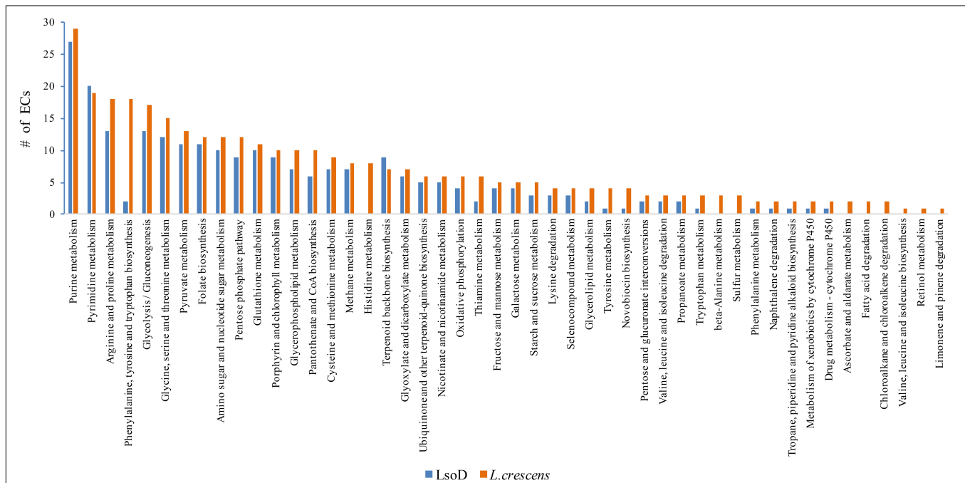
FIGURE 5 | Comparison of the number of ECs for LsoD and L. crescens is mapped to metabolic and degradative pathway. The absolute number of ECs for each pathway is graphically represented.
