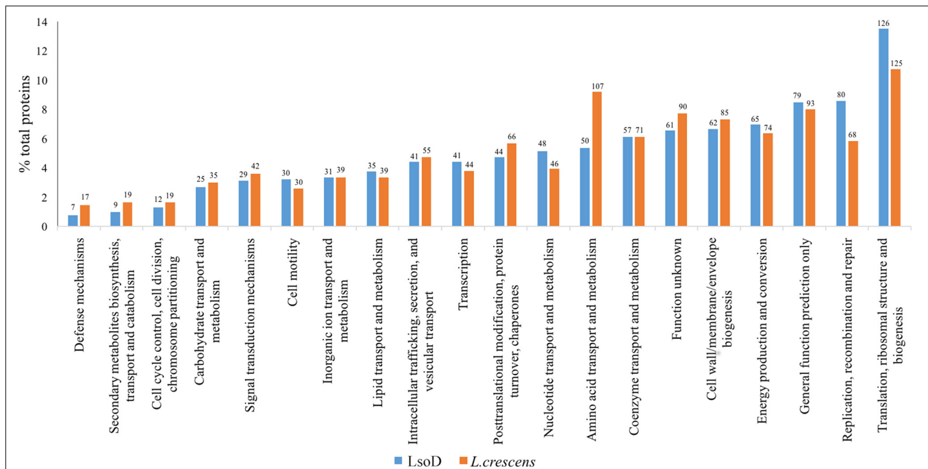
FIGURE 4 | Comparison of clusters of orthologous groups (COGs) assignments determined by the WebMGA server of LsoD and L. crescens are plotted as a percentage of their total respective genomes. The absolute number of genes is indicated above each bar.
