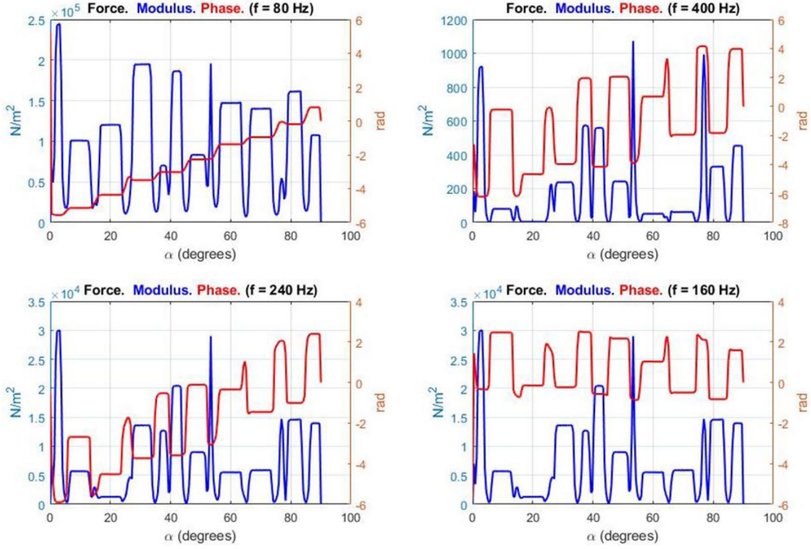
Fig. 5 Alternating force components obtained with the parameters f = 40 Hz, s = 2.5 %, I_p = 3 A, f_h = 5 \times 40 Hz, s_h = 80.50 %, I_{ph} = 3/5 A, \gamma = 1 degree (linear B–H model)
