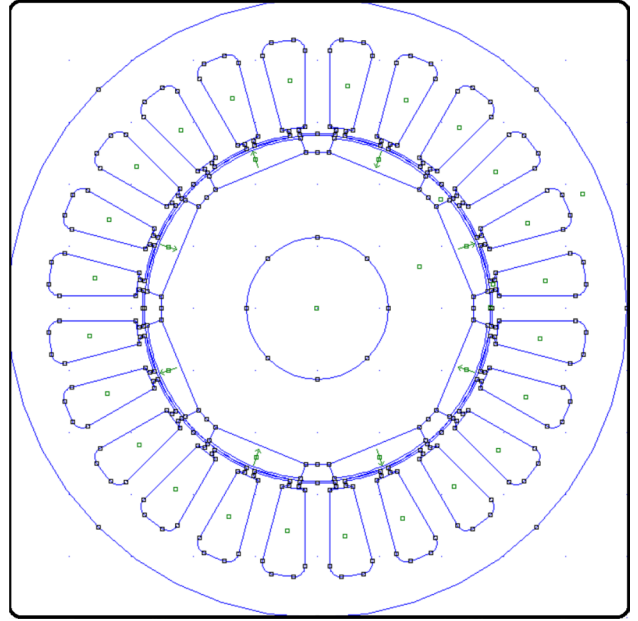
Fig. 2 Brushless machine: complete geometry drawn in FEMM software
