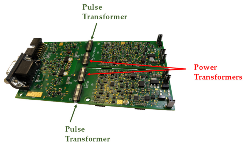
Figure 6. Gate driver card for two semiconductors with four designated planar transformers.
