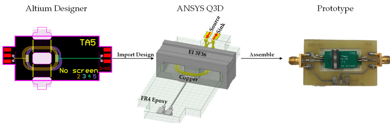
Figure 11. Pulse transformer design analysis in Altium Designer and ANSYS Q3D.
