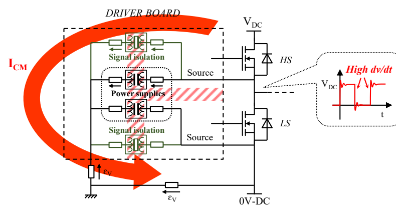
Figure 7. Common-mode current routing through isolated signal transformers on gate driver board.
