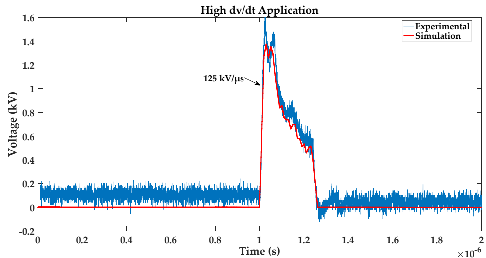
Figure 16. Experimental vs. simulated high dv/dt application.
