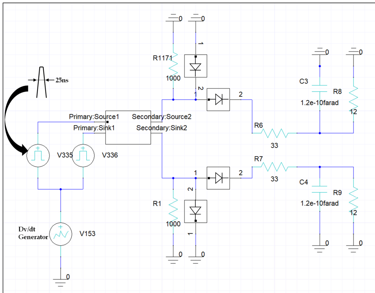
Figure 14. Sustainability of planar transformer to 125 kV/ \mu s dv/dt simulated in ANSYS Circuit Design.
