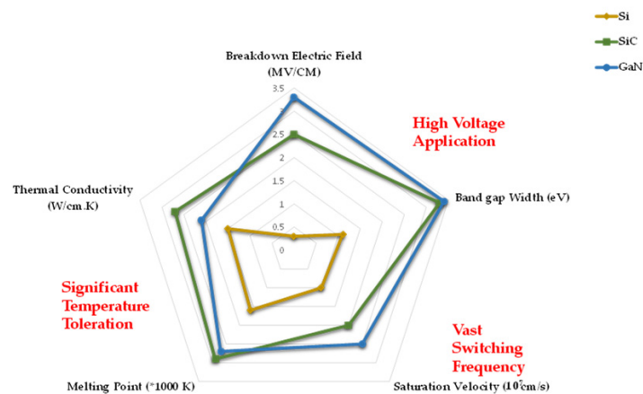
Figure 3. Intrinsic properties of particular semiconductor materials: Si, SiC, GaN.
