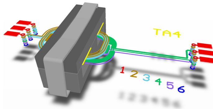
Figure 5. An example of a planar transformer with an EI core.
