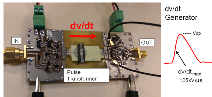
Figure 15. Experimental evaluation of typical shielded pulse transformer toleration to high dv/dt.
