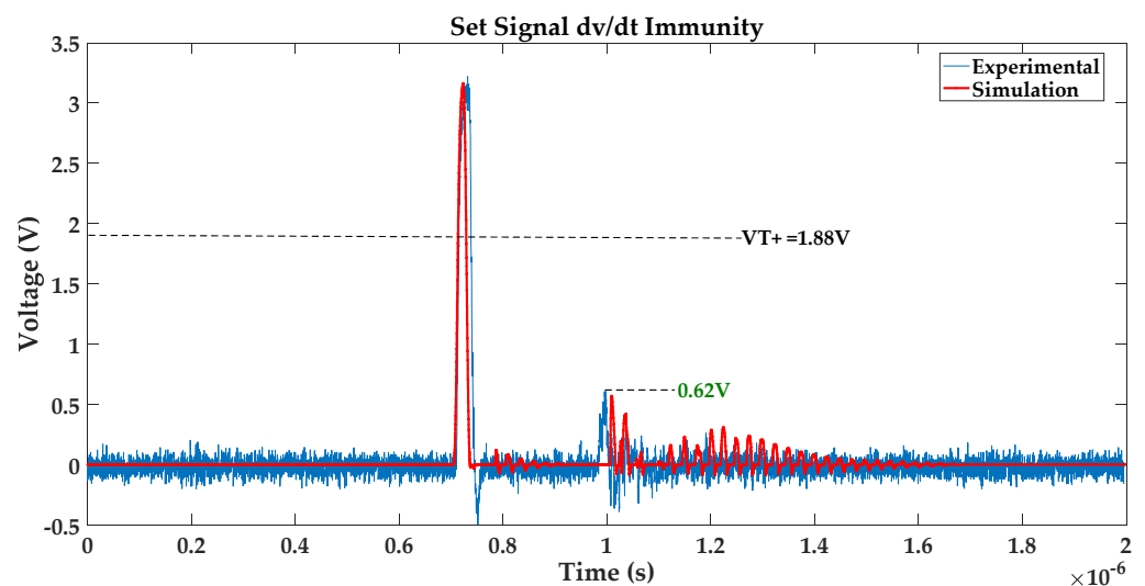
Figure 17. Experimental vs. simulated dv/dt immunity of a typically shielded transformer.
