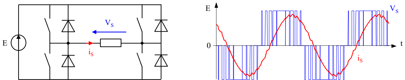
Figure 1. Single-phase full bridge inverter and its associated waveform.
