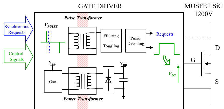
Figure 8. Principle of data signal transmission through a gate driver.
