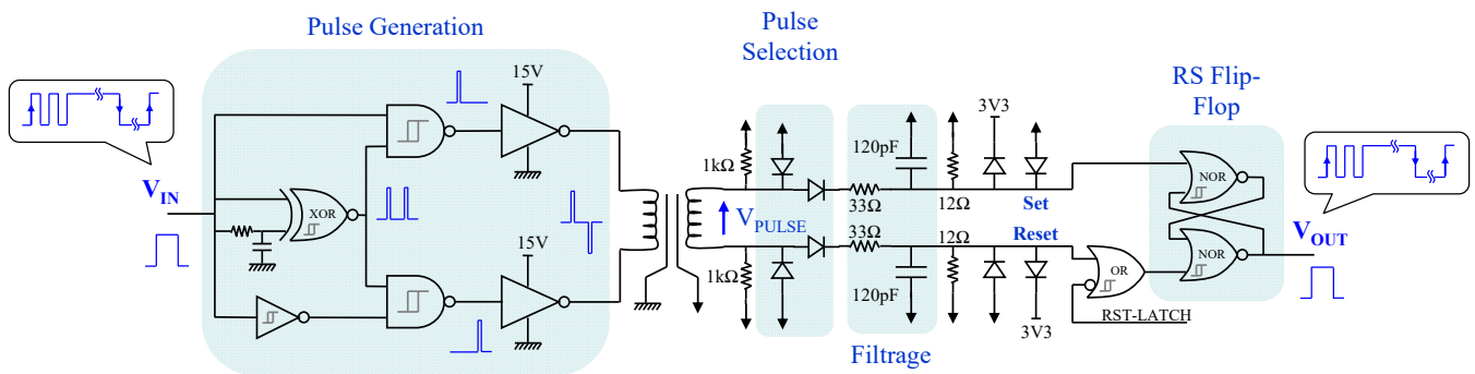
Figure 12. Pulse generation and transmission electronic circuit.
