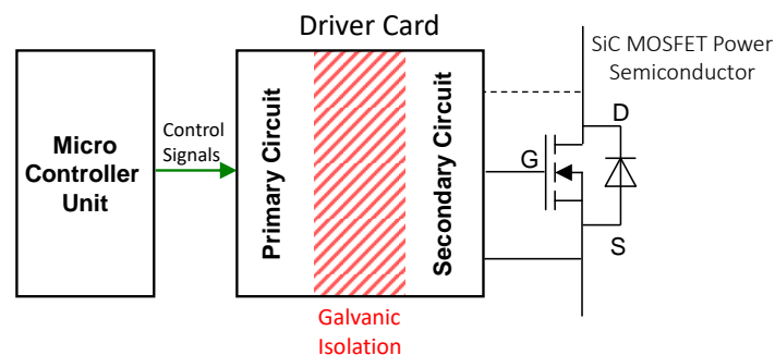
Figure 4. Generic demonstration of gate driver card assemblage.
