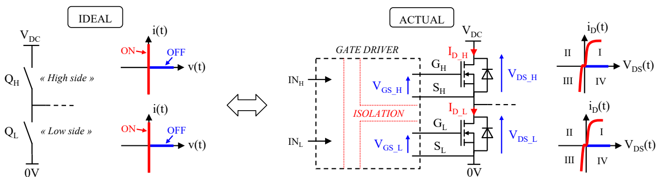
Figure 2. A fundamental example of a switching N-MOSFET cell.
