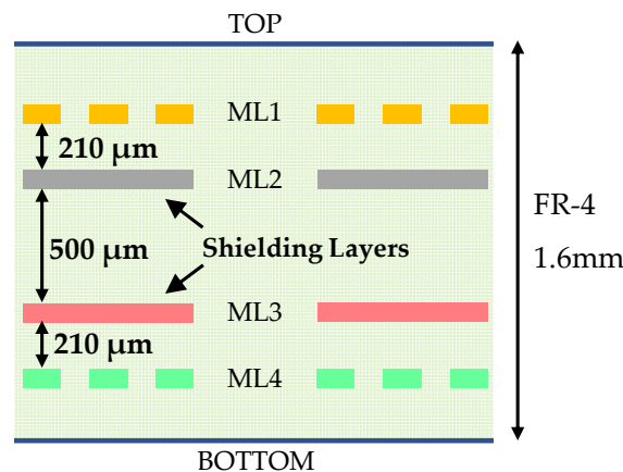
Figure 13. Pulse transformer section view.
