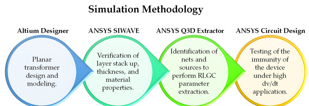
Figure 10. Simulation methodology process followed to analyze pulse transformers.
