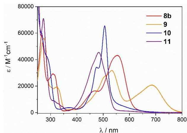
Figure 4. Electronic absorption spectra of 8b in acetonitrile and its different protonation species: 8b ( \epsilon^{554} = 43\,000 M^{-1}cm^{-1} ), 9 ( \epsilon^{686} = 21\,000 M^{-1}cm^{-1} , \epsilon^{533} = 32\,000 M^{-1}cm^{-1} ), 10 ( \epsilon^{506} = 66\,000 M^{-1}cm^{-1} ), 11 ( \epsilon^{483} = 45\,000 M^{-1}cm^{-1} ).
