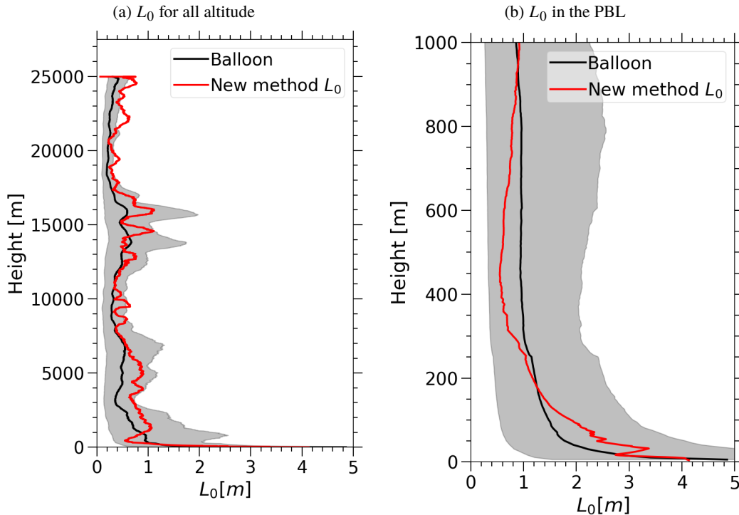
Figure 6: Comparison of the mean vertical profiles of the L_0 deduced from radiosounding in black and estimated using our new method in red. Grey colored surface shows the interval between the first and the third quartiles of radiosounding data. (a) for all altitude and (b) a zoom at the planetary boundary layer.
