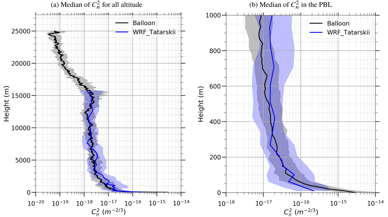
Figure 5: Comparison of the vertical profiles of the C_n^2 deduced from radiosounding (black) and using WRF_Tatarskii model (blue). Thick lines indicate the median value and shading show the interval between the first and the third quartiles. (a) for all altitude and (b) a zoom at the planetary boundary layer.
