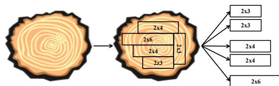
Fig. 1. The sawing of a log into lumbers is a diverging process with co-production. (Morin et al., 2015)
