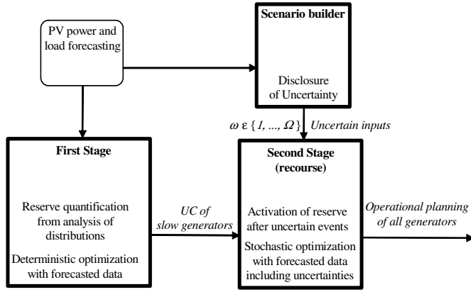
FIGURE 7. Sequence of the two-stage stochastic programming for the reserve and energy optimization function.
