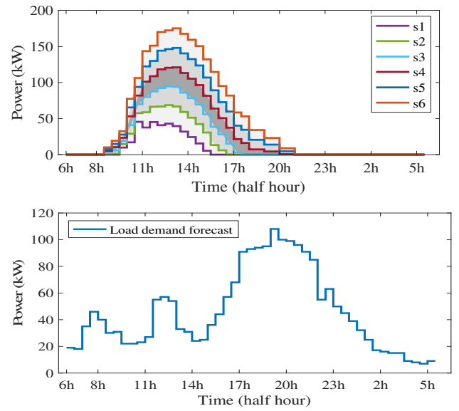
FIGURE 16. Expected PV generation under six probable scenarios and forecasted load demand.
