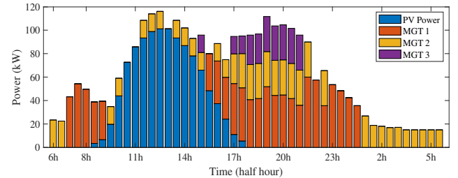
FIGURE 17. Generation scheduling under stochastic optimization.
