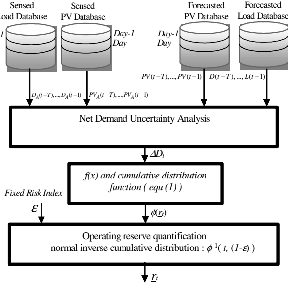
FIGURE 4. Scheme of the risk-constrained probabilistic method for reserve determination
