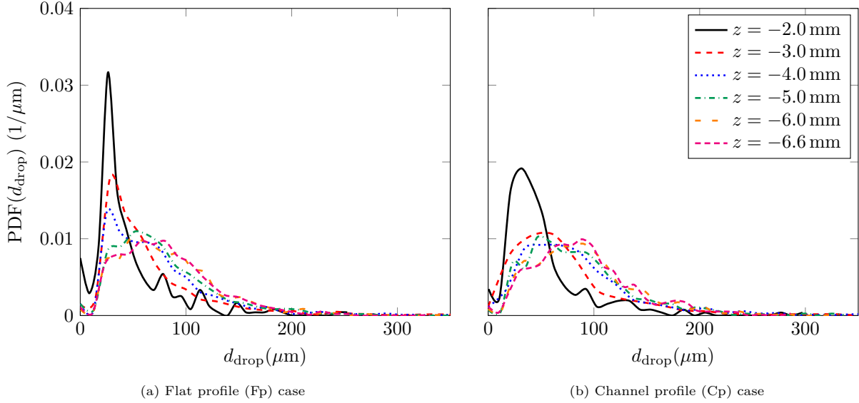
Figure 16: PDF of DSD sampled at various downstream locations of z = -2 mm (—), -3 mm (---), -4 mm (·····), -5 mm (-.-.-), -6 mm (- - -), -6.6 mm (- - -) from flat profile (Fp) and channel profile (Cp) simulation cases.
