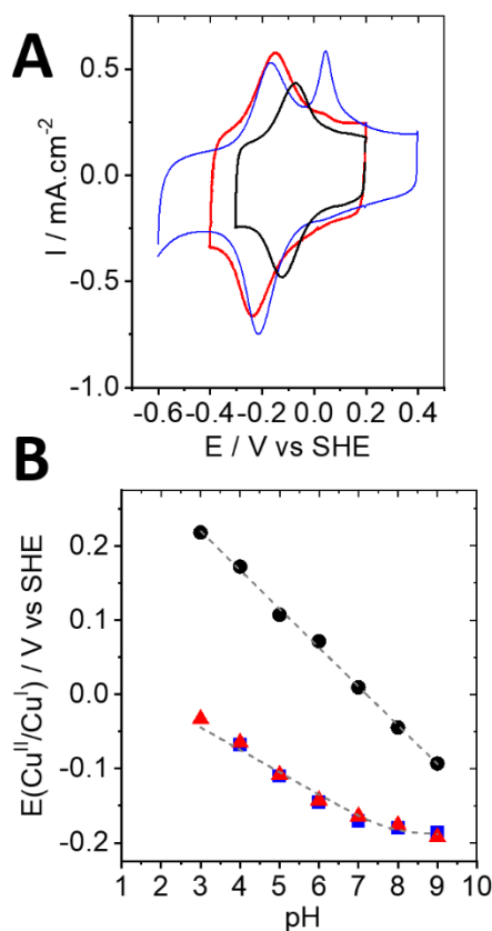
Figure 2. (A) CVs of [Cu(CF 3 PMP tBu -pyrene)] (black), [Cu(MePMP-pyrene)] (red) and [Cu(HPMP-pyrene)] (blue), (straight line) immobilized on the MWCNT electrode collected at pH 9 (0.1 M Britton Robinson buffer) under argon ( v= 10 \text{ mV s}^{-1} ) ; (B) Corresponding experimental and fitted (gray dashed line) evolution of the redox potential of the Cu II /Cu I redox couple for as a function of the pH for of [Cu(CF 3 PMP tBu -pyrene)] (●), [Cu(MePMP-pyrene)] (▲) and [Cu(HPMP-pyrene)] (■), The geometrical surface of the electrode (0.07 cm 2 ) was used to calculate current densities.
