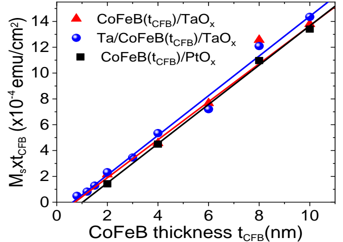
Fig. 1. Saturation magnetic moment per unit area versus thickness of the CoFeB-based systems annealed at 225° C. Symbols refer to experimental data and solid lines are linear fits.
