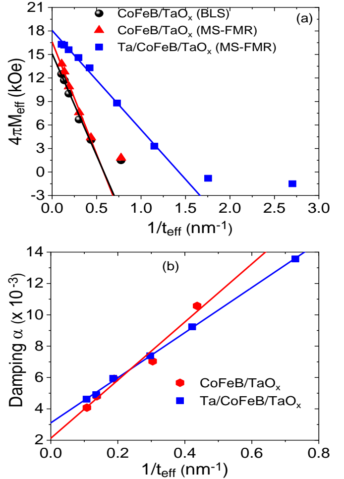
Fig. 2. (a) Effective magnetization ( 4\pi M_{\text{eff}} ) and (b) Gilbert damping constant as a function of the inverse effective thickness of CoFeB films for CoFeB/TO x and Ta/CoFeB/TO x systems. 4\pi M_{\text{eff}} values have been extracted from the fit of the in-plane applied magnetic field dependence of spin waves frequency measured by MS-FMR and BLS. Symbols refer to experimental data and solid lines are linear fits.
