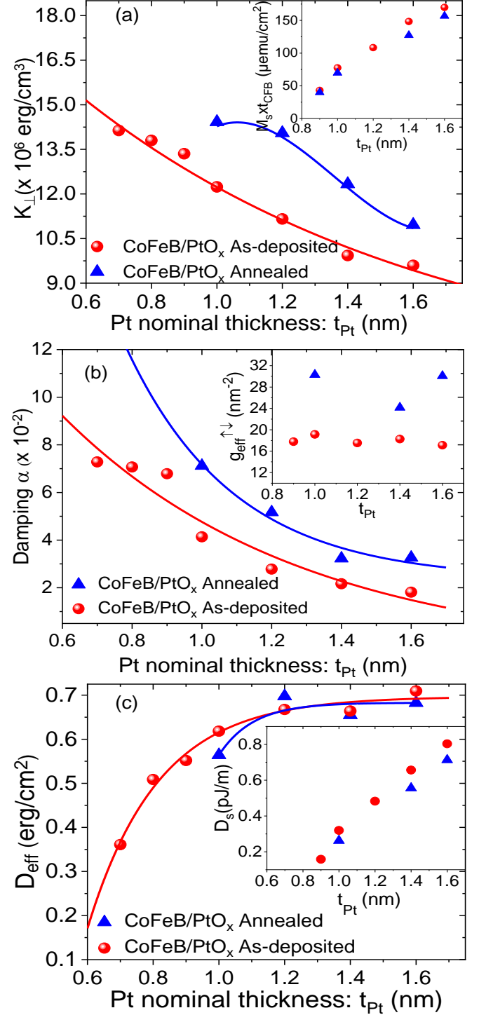
Fig. 3. Variations of (a) perpendicular anisotropy constant (K ⊥ ), (b) Gilbert damping and (c) effective iDMI constant (D eff ) as a function of the nominal Pt thickness (t Pt ) for the as grown and the 225 °C annealed CoFeB(1.5 nm)/PtO x films. PtO x is obtained by oxidation of Pt t Pt indicated in the horizontal axis. Symbols refer to experimental data and solid lines are eye guides. Insets show (a) areal magnetic moment, (b) effective spin mixing conductance and (c) surface iDMI constant versus t Pt .
