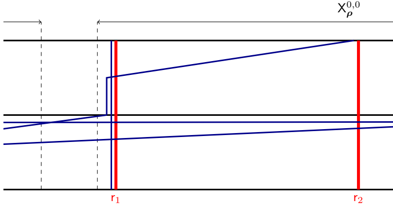
FIGURE 2. Focusing on the orange rectangle of Figure 1
