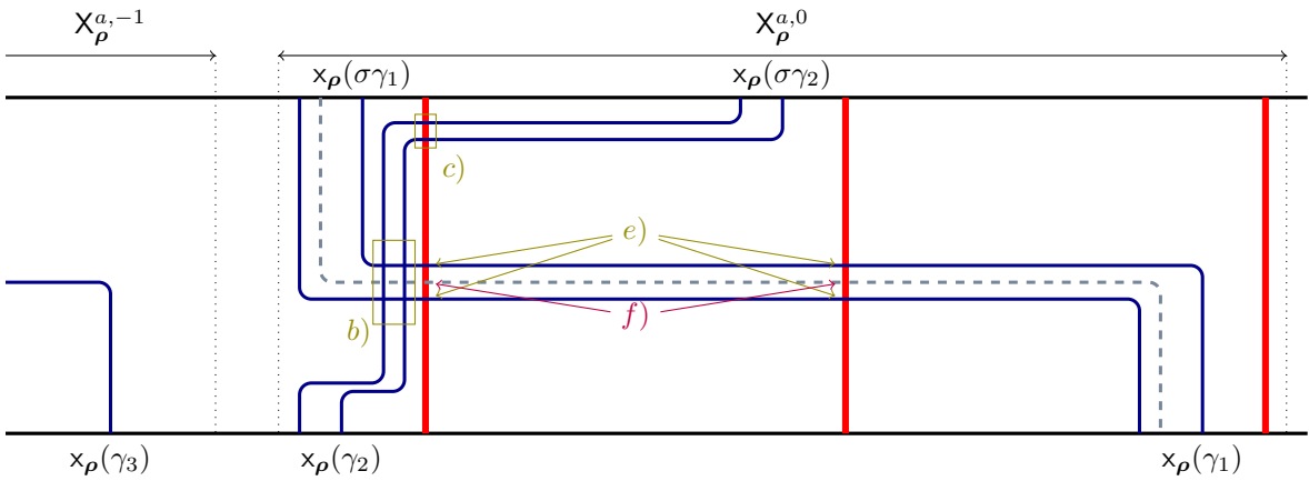
FIGURE 4. Illustration of Proposition 4.38 for a diagram B_\lambda^{[1]}
