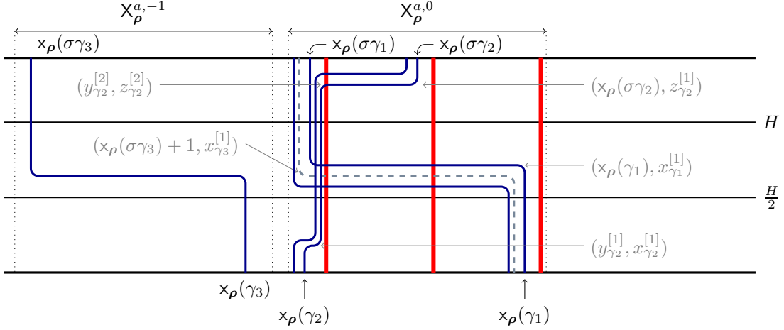
FIGURE 3. Illustration of a diagram B_\lambda^{[1]}
