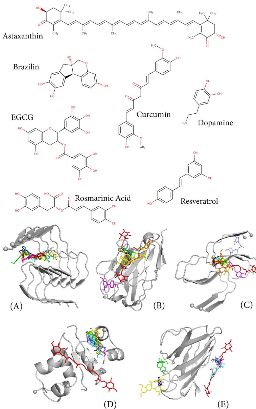
Figure 31. Chemical structures and the binding poses of the seven natural ligands to (A) 4Aβ 11-42 peptides (PDB 2MX), 911 (B) αS (2X6M) 912 , (C) hIAPP (6Y1A) 253 , (D) insulin (1GUJ) 913 and (E) SOD1 (6FLH). 914 Binding poses were obtained by Autodock vina 915 with exhaustiveness of 8 and a grid of 60 × 60 × 60 Å covering the whole receptor. 916 Astaxanthin, brazilin, curcumin, dopamine, EGCG, resveratrol, and rosmarinic acid are highlighted in red, green, light blue, blue, yellow, magenta, and orange colors, respectively. The authors designed the figure.
