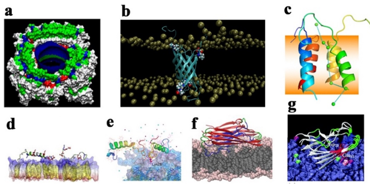
Figure 19. Different interaction models of full-length A \beta_{40/42} peptides with lipid membranes. (a) A \beta transmembrane pores with high Ca ^{2+} permeability and selectivity. 579 (b) Tetrameric A \beta_{42} \beta -Barrel pores in PC/PS/cholesterol/sphingomyelin and DPPC bilayers 591 . (c) Tetrameric A \beta_{42} \alpha -helix-bundle pores in DPPC bilayer with Ca ^{2+} transport across the bilayer 596 . (d) A \beta_{42} monomer with both \alpha -helical and \beta -structure conformations being adsorbed on cholesterol-rich POPC bilayers, where increase of cholesterol promotes A \beta -membrane interactions and adsorption 603 ; (e) A \beta dimers on the GM1-clustering membrane, with C-terminal residues be inserted into membrane 604 ; (f) A \beta tetramers with typical U-bent \beta -structure being preferentially adsorbed on and inserted into POPE bilayer over POPC bilayer, as driven by electrostatic interactions 609 ; (g) A \beta_{42} pentamer being adsorbed onto POPC/POPG bilayer via Ca ^{2+} ionic bridges between Glu22 and Asp23 and anionic headgroups of the lipid bilayer. 610 The authors design the figure from the above references.
