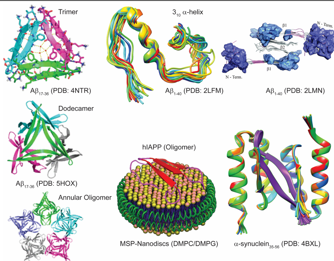
Figure 7. High-resolution structures of amyloid oligomers in solution or membrane-bound state solved using X-ray and NMR methods, the exception being the model of A\beta_{40} assembly toxic surface (top, right). The figure was designed by the authors.
