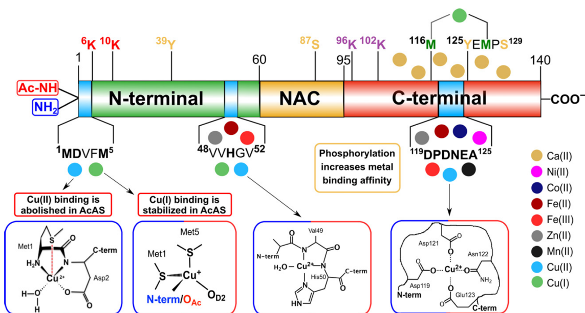
Figure 28. Metal binding sites and post-translational modifications of \alpha S. \alpha S harbors three binding sites for metal ions (displayed with colored circles): the low affinity, non-specific metal binding site at the acidic DPDNEA segment in the C-terminal, the His50 site, and the first five residues at the N-terminal. His50 can anchor transition-metal ions such as Zn(II), Fe(III), and Fe(II), but the highest affinity is found for Cu(II) and Cu(I) ions. The N-terminus of \alpha S is a high affinity and highly specific site for Cu ions. This figure is reproduced from Ref. 734.
