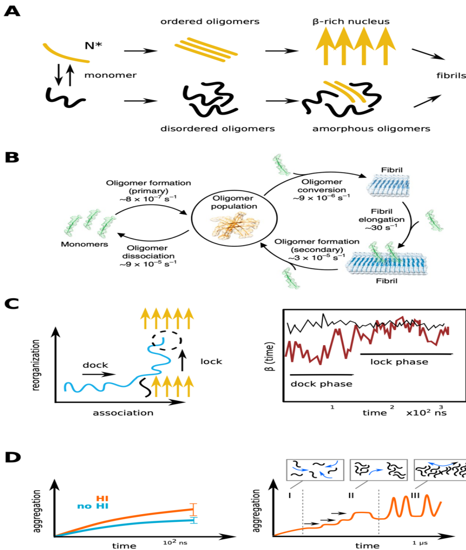
Figure 11. Panel A: Schematic representation of two extreme scenarios, the one-step and the two-step nucleation process for early steps of amyloid aggregation. Panel B: Characteristic steps and kinetics of A \beta 42 amyloid proliferation determined experimentally, with the reaction rates at a concentration of 5 \mu\text{M} 370 . Panel C: Description of the dock and lock mechanism, left chart schematically reproduces the results, 375 where the evolution of the \beta -structure of a monomer is followed in time during the dock and lock phases. Panel D: Effect of hydrodynamic interactions on the aggregation process of A \beta 16-22 peptides (left) and protofibril elongation due to oligomer fusion (right) as observed in LBMD simulations. 366,394 The authors designed panel A, panels C and D are updated from 366, 375 and 394 . Panel B was taken from 370 .
