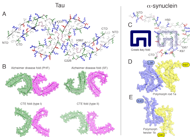
Figure 5. Orthogonal view of the three-dimensional structural models of tau filaments and \alpha -synuclein amyloid fibrils. NTD and CTD are the N-terminal and C-terminal domain. (A) Solid-state tau paired PHF spanning residues 306-378 in the right protofilament. (B) Cryo-EM PHF and SF tau amyloid cores in AD. In chronic traumatic encephalopathy (CTE), tau filaments contain predominantly the type I (90%) and type II filaments. The inter-protofilament interfaces are different compared to those in AD. (C) Amyloid core of human \alpha -synuclein amyloid fibrils (PDB entry 2n0), containing a Greek-key fold. (D-E) amyloid core fibril structure of \alpha -synuclein: polymorph rod 1a (PDB entry 6CU7) and polymorph twister 1b (PDB entry 6CU8). The authors prepared this figure with pymol 254 .
