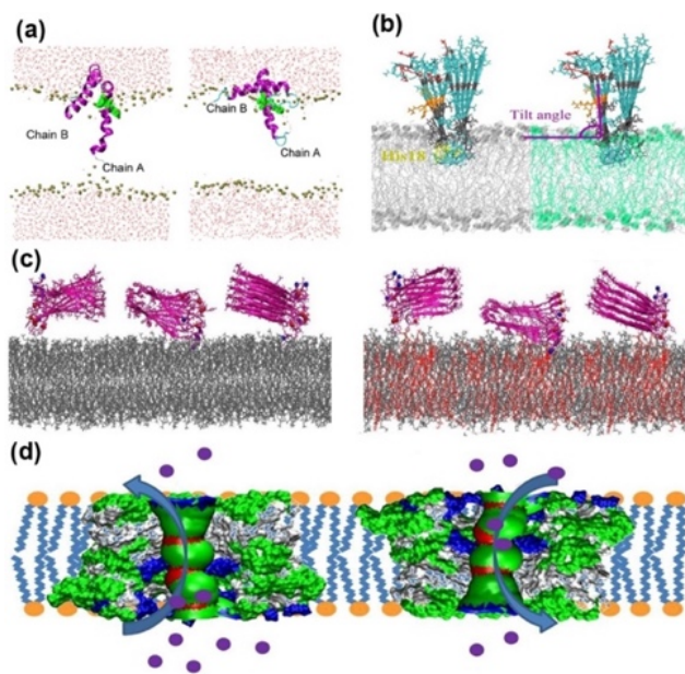
Figure 21. Different interaction models of full-length hIAPP 1-37 oligomers with lipid membranes. (a) hIAPP dimers with \alpha -helical structure insert into POPG bilayers with different insertion depths, strongly depending on interactive contacts of hIAPP dimers with POPG bilayers 621 ; (b) hIAPP pentamer with U-bent \beta -structures to be partially inserted into (left) DPPG and (right) DPPC/DPPG bilayers via the turn region 629 ; (c) hIAPP pentamer with U-bent \beta -structures to be adsorbed on (left) POPC and (right) POPG/POPE bilayers with different hIAPP orientations 613 ; (d) double hIAPP pores with different (left) a “turn-to-tail” and (right) a “tail-to-turn” orientations in DOPC bilayers to show nonselective, ion-permeable activity 632 . The authors design the figure.
