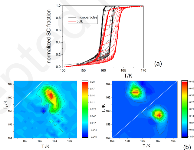
Figure 7. (a) Superposition of the First-order reversal curves in the heating mode for in-BuOH embedded [Fe III (3-OMeSalEen) 2 ]PF 6 bulk (red) and 8 μm-long (black) particles. The samples were previously cycled and brought out in the stable hysteretic regime ( d , sweeping rate = 0.2 Kmin -1 ). The FORC plots recorded in the two branches of the major hysteresis show a zero slope at any reversal temperature; (b) Corresponding FORC distributions in the heating mode for bulk (left) and in both modes for 8 μm-long particles (right).
