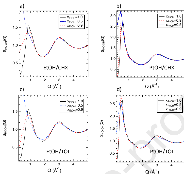
Figure 4. Partial structure factor ( S_{HO-OH}(Q) ) of EtOH/CHX a), PtOH/CHX b), EtOH/TOL c), PtOH/TOL d) as a function of the molar fraction of alcohol.
