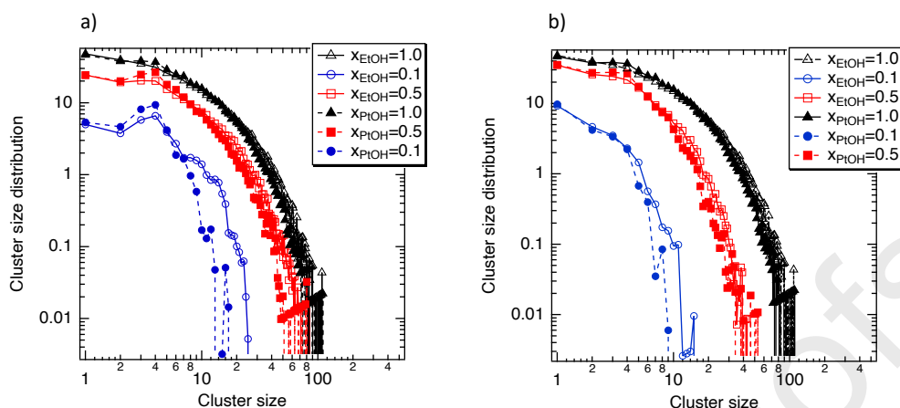
Figure 5. Cluster size distribution as a function of molar fraction of alcohol in CHX a) and TOL b) mixtures.
