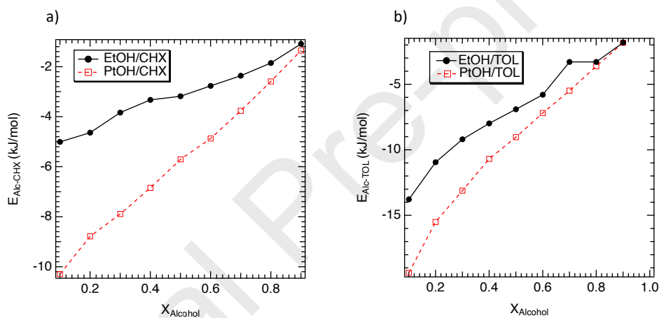
Figure 6. Calculated energy between the alkyl chain of alcohol molecules and CHX a) and TOL b) as a function of the molar fraction of alcohol.
