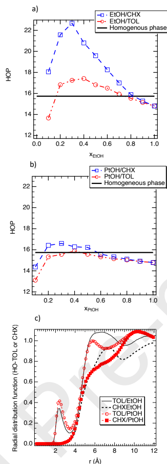
Figure 2. HOP of EtOH a) and PtOH b) for both TOL and CHX binary mixtures as a function of the molar fraction of alcohol. The average uncertainties about the HOP are around 0.8. c) Radial distribution functions between the hydrogen atoms of OH groups of EtOH and PtOH and the centre of mass of toluene molecules in both CHX and TOL mixtures at x_{Alcohol}=0.5 .
