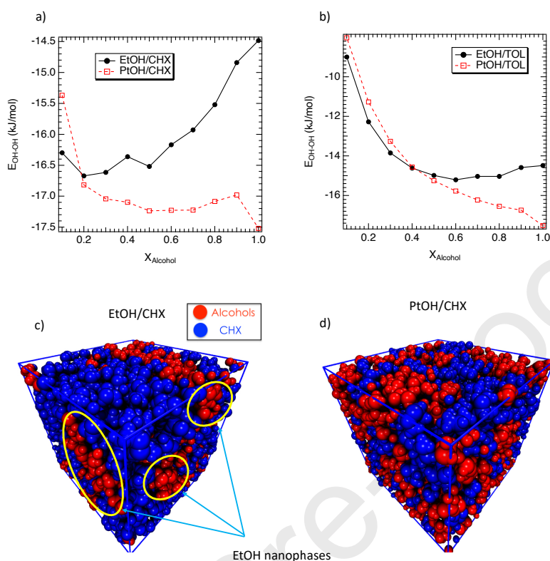
Figure 3. Calculated energy between the OH groups of alcohol molecules as a function of the molar fraction of alcohol into the CHX a) and TOL b) mixtures. Snapshots of EtOH/CHX c) and PtOH/CHX d) at x_{Alcohol}=0.5 .
